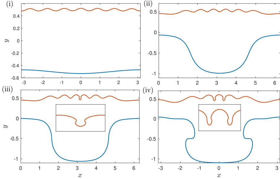
Figure 17: Four typical wave profiles with R_1 = 1.01 , R_3 = 0.95 , h_1 = 1 , h_3 = 1 , and k = 1 .
