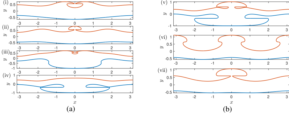
Figure 12: Almost limiting wave profiles corresponding to the labelled solutions (i) to (vii) in figure 11.
