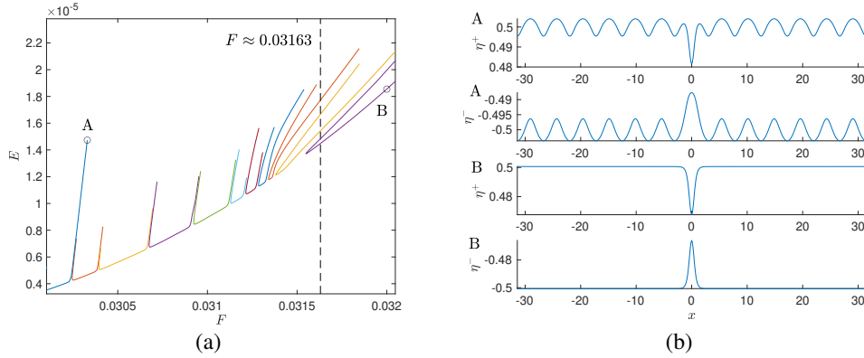
Figure 16: (a) Speed-energy bifurcations of mode-2 waves with R_1 = 1.01 , R_3 = 0.99 , h_1 = h_3 = 0.1 , and k = 0.1 . The black dashed line represents the max phase speed of mode-1 waves. (b) Solutions A and B labelled in (a).
