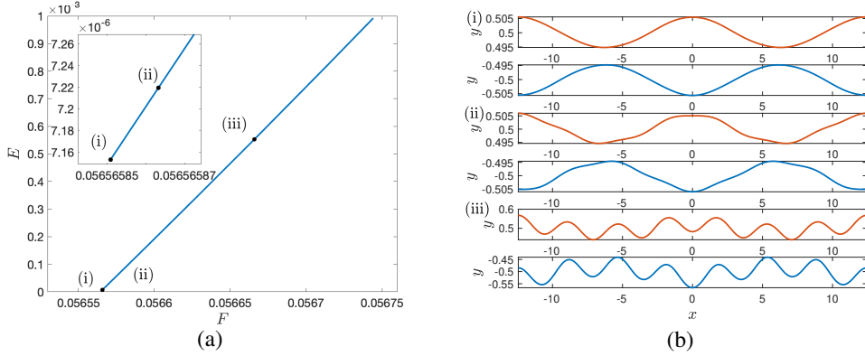
Figure 8: (a) Speed-energy bifurcation curves with R_1 = 1.01 , R_3 = 0.99 , h_1 = 1 , h_3 = 1 and k = 0.2525 . (b) Three typical wave profiles corresponding to the labelled solutions in (a). The red and blue curves are the upper and lower interfaces.
