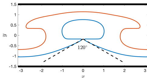
Figure 4: Almost limiting wave profile (iii) in figure 3(c) in one spatial period. The black dash line represents the limiting 120^\circ angle.
