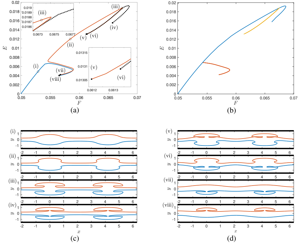
Figure 5: Numerical solutions of mode-2 waves with R_1 = 1.01 , R_3 = 0.99 , h_1 = 1 , h_3 = 1 , k = 1.5 . (a) Speed-energy bifurcation branches of the Euler case. (b) Speed-energy bifurcation branches of the Boussinesq case. (c, d) Typical wave profiles of Euler case which are labelled in (a) and plotted in two spatial periods.
