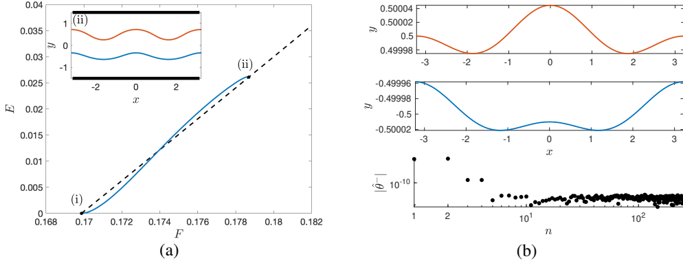
Figure 7: (a) Speed-energy bifurcation curves with R_1 = 1.1 , R_3 = 0.9 , h_1 = 1 , h_3 = 1 , k = 0.97651 (blue, mode-2), and k = 1.953 (black, mode-1). The energy of the mode-1 waves are calculated in two spatial periods. The figure in the upper left box shows the wave profile of solution (ii). (b) The top and middle figure are the upper and lower interfaces of solution (i) in (a). The bottom figure displays the absolute value of \hat{\theta}^- of solution (i) in a log-scale, where \hat{\theta}^- is the Fourier coefficient of the lower interfacial inclination angle \theta^- , and n is the order of the Fourier modes.
