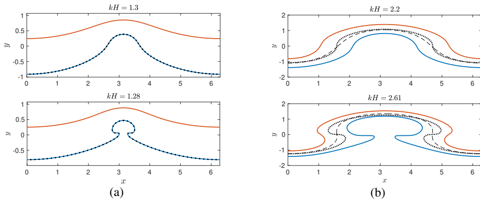
Figure 2: (a) Typical wave profiles of R_1 = 10 , R_3 = 1 , h_1 = 100 , h_3 = 99 and k = 1 . The upper and lower interfaces are the solid curves. Due to the chosen parameters, the upper curve is the real interface of a two-layer system and the lower curve is a streamline. The black dots are solutions of the corresponding two-layer deep water system with density ratio 0.1. (b) Typical wave profiles of R_1 = 1.01 , R_3 = .99 , h_1 = 99.5 , h_3 = 99.5 and k = 1 . The black dashed lines denote the mid streamlines of three-layer solutions. The black dots are solutions of the corresponding two-layer deep water system with density ratio 0.9802. In (a) and (b), H denotes the crest-to-trough wave amplitude of the blue curve.
