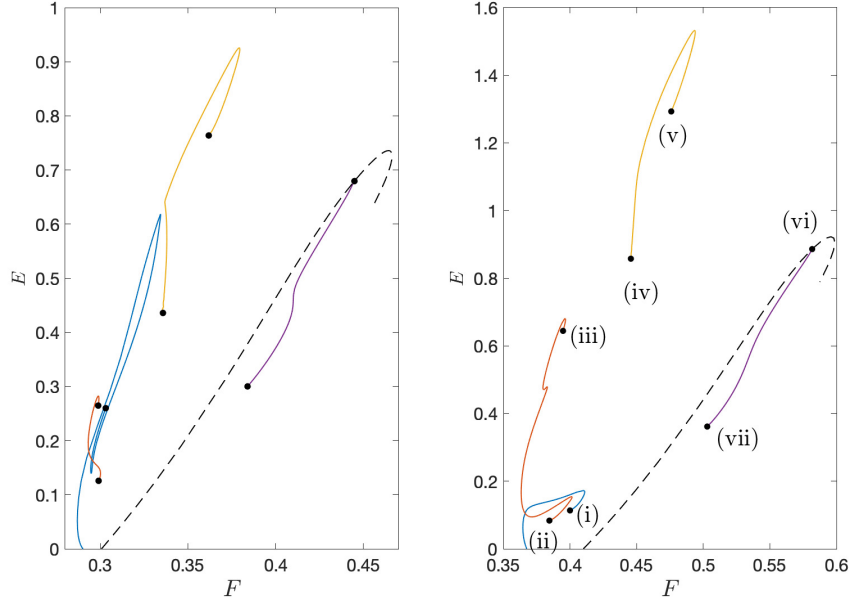
Figure 11: Left: Speed-energy bifurcation curves of the mode-2 waves with R_1 = 1.3 , R_3 = 0.7 , h_1 = 1 , h_3 = 1 , and k = 1 . Right: Speed-energy bifurcation curves of the mode-2 waves with R_1 = 1.5 , R_3 = 0.5 , h_1 = 1 , h_3 = 1 , and k = 1 . The black dashed curve is the bifurcation of the mode-1 waves with the same parameters except k = 2 . The corresponding energy is calculated in two spatial periods.
