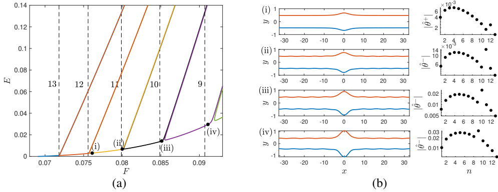
Figure 13: (a) Speed-energy bifurcation curves for R_1 = 1.01 , R_3 = 0.99 , h_1 = 50 , h_3 = 50 , and k = 0.096 . The vertical dashed lines denote the predicted value of F where the mode-2 waves are resonant with the mode-1 waves having waves number nk . The corresponding values of n are shown close to the vertical lines. (b) Typical wave profiles and related absolute value of one of \hat{\theta}^\pm of the labelled solutions (i) to (iv) in (a), where \hat{\theta}^- and \hat{\theta}^+ are the Fourier coefficients of the inclination angle of the lower and upper interface.
