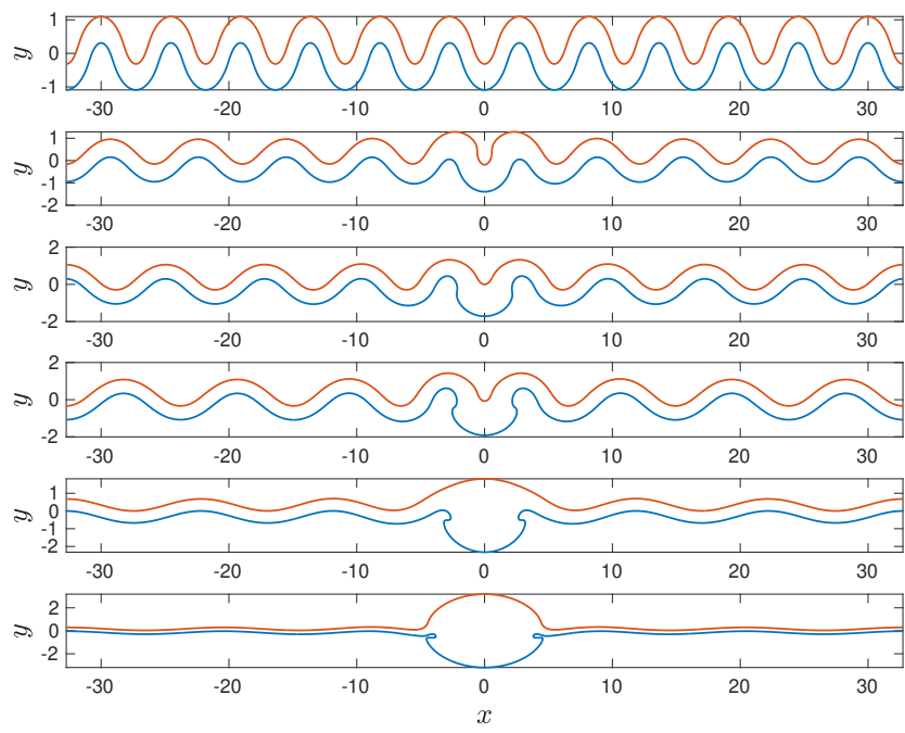
Figure 15: Six different (almost) limiting wave profiles with R_1 = 1.01 , R_3 = 0.99 , h_1 = 50 , h_3 = 50 , and k = 0.096 .
