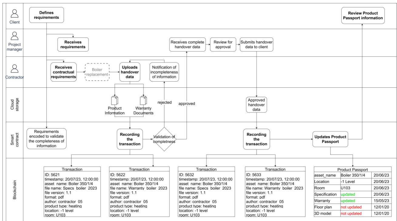
Figure 3. A conceptual blockchain framework of handover information collection process.
