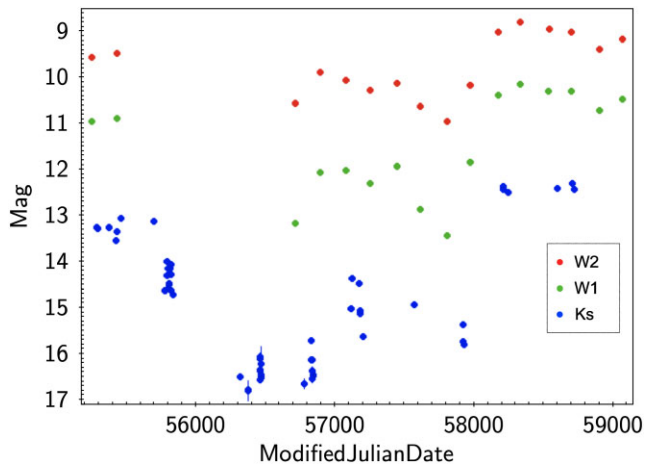
Figure E3. VVV and WISE/unTimely light curves of the dipping YSO source 28 in K_s (blue), W1 (green) and W2 (red).
