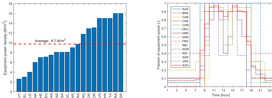
Figure 3: Office occupant density values and schedules provided by the reviewed codes
