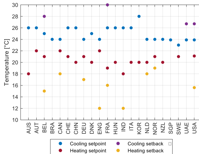
Figure 4: The heating and cooling setpoint and setback temperatures in the reviewed codes. Absence of points on the graph mean setpoints are not specified (i.e., the equipment can be turned off).
