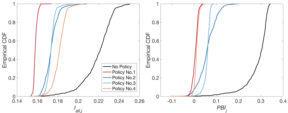
Figure 3. Empirical cumulative distribution functions (CDF) of I_{all,j} (left panel) and PBI_j (right panel), for the 500 sets of GMFs. Results are shown for policies No.1 to 4 (and no policy).
