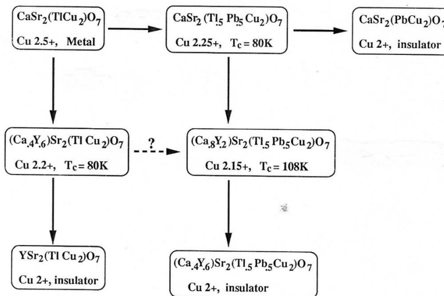
Figure 1. The chemical control of High Temperature Superconductivity in the septenary cuprates [4, 5]; illustrated from the original data by W Y Liang ( Cambridge University )
