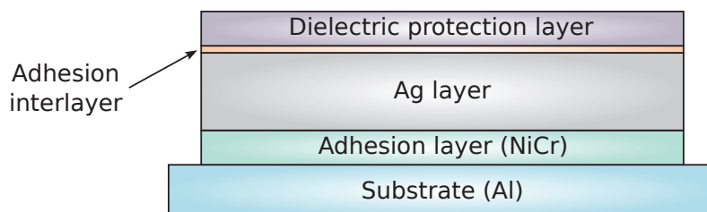
Figure 2. Indicative structure of the multilayer coating stack. The total coating tickness is approximately 350 nm.
