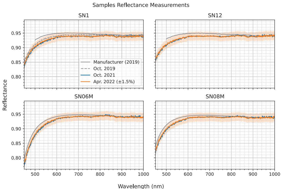
Figure 5. Reflectance measurements of four coated samples performed with two different setups, by the manufacturer and by the authors. One comparison measurement of sample SN1 (dashed gray line) was performed sufficiently close in time to the manufacturer’s measurement to be useful to assess the cross-calibration of the two setups, which appear to have a bias.
