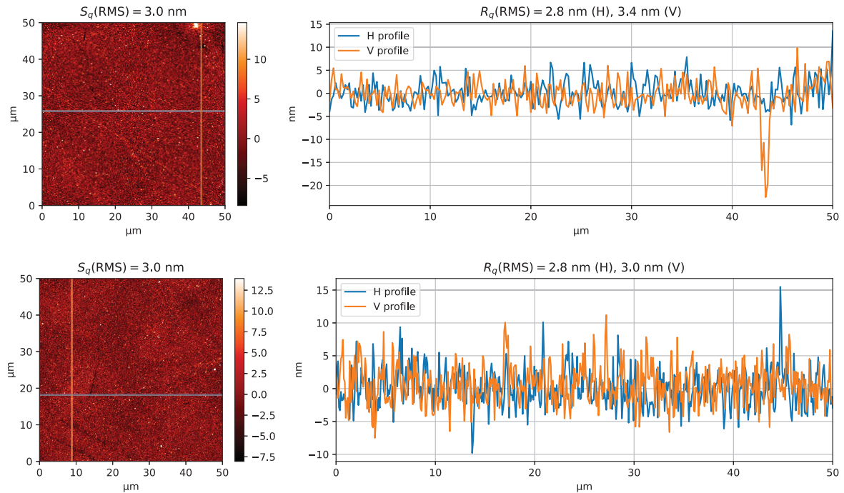
Figure 7. AFM scans (left) of sample SN06M before (top) and after (bottom) the storage period. For each scan, two line profiles are also provided (plots on the right). The two scanned areas do not necessarily coincide.
