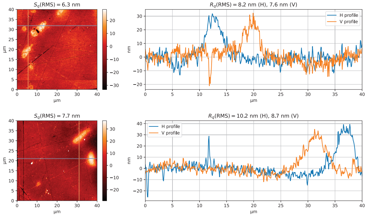
Figure 6. AFM scans (left) of sample SN01 before (top) and after (bottom) the storage period. For each scan, two orthogonal line profiles are also provided (plots on the right). The two scanned areas do not necessarily coincide.
