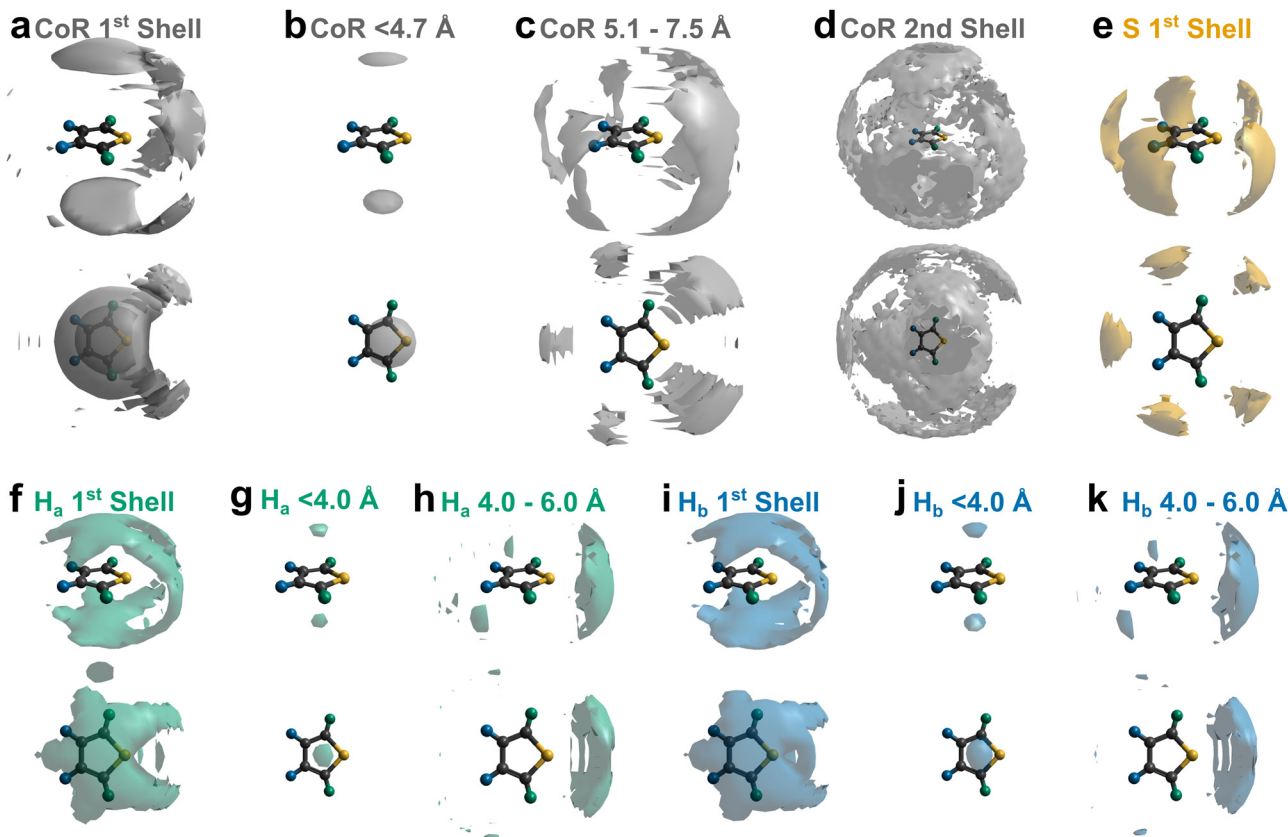
Fig. 5 (a)–(d) SDFs highlighting most likely 10% position of the CoR of adjacent thiophene molecules in (a) the first solvation shell, \leq 7.5 Å, (b) < 4.7 Å, (c) 5.1–7.5 Å, and (d) second solvation shell (7.5–12.1 Å). (e)–(k) SDFs highlighting most likely 5% of positions of atomic sites [(e), S; (f)–(h), H a ; (i)–(k), H b ] of adjacent thiophene molecules at various distances: (e), (f), and (i) the first solvation shell; \leq 7.5 Å, (g) and (j) < 4.0 Å; (h) and (k) 4.0–6.0 Å. Additional 1 st shell CoR SDFs provided at various percentage most likely positions provided in ESI, † Fig. S1.
