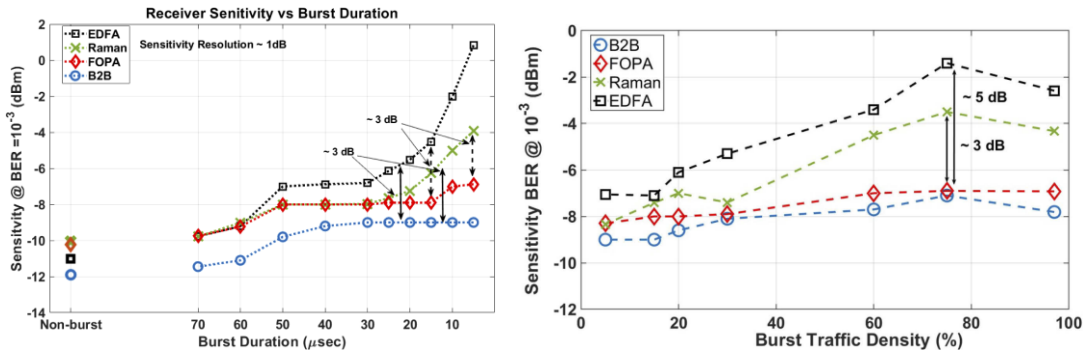
Figure 6. Receiver sensitivity for each tested amplifier for fixed burst period of 100 \mu s and variable burst duration (left), and for fixed burst duration of 30 \mu s and variable burst traffic density (right).
