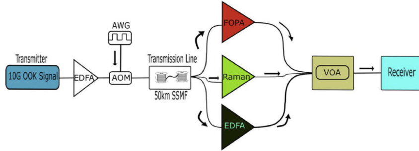
Figure 5. Testbed for comparison of PI-FOPA, EDFA and discrete Raman amplifier in extended PON architecture when amplifying burst traffic.
