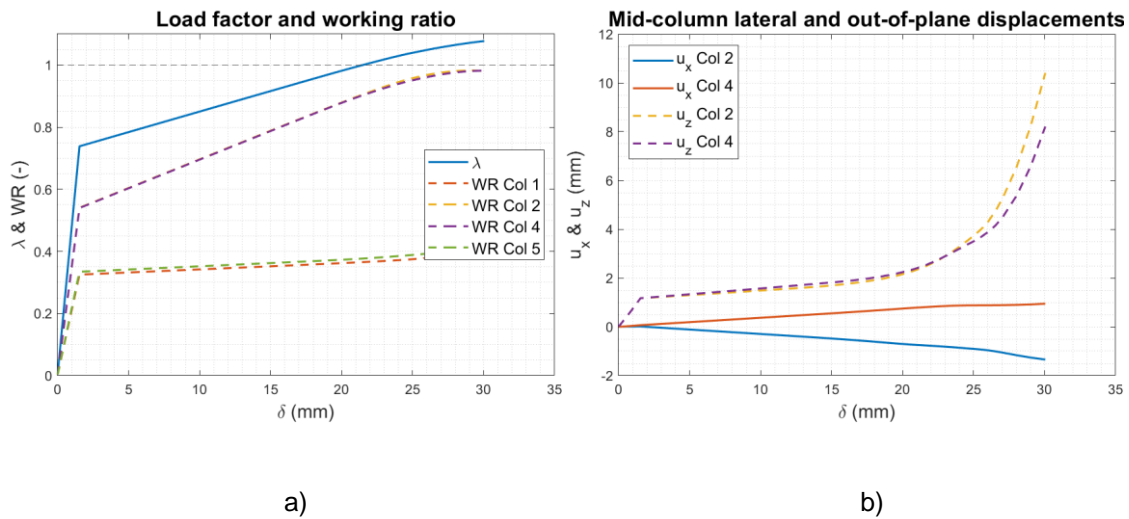
Figure 5. Results for the structure retrofitted with the roof-truss: (a) load factor ( \lambda ) and work ratio (WR) of columns at the 1 st storey, (b) horizontal displacements of columns' middle nodes ( u_{Col} ).
