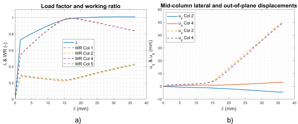
Figure 6. Results for the structure retrofitted with bracings at the 2 nd storey: (a) load factor ( \lambda ) and work ratio (WR) of columns at the 1 st storey, (b) horizontal displacements of column's middle nodes ( u_{Col} ).
