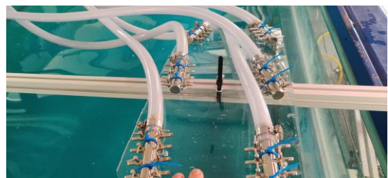
(B) 8 way manifolds to feed each of the 96 nozzles
