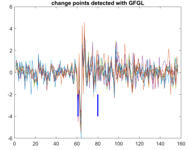
(i) The change points identified with \lambda_1 = 0.5 and \lambda_2 = 60 are \{61, 80\} .
