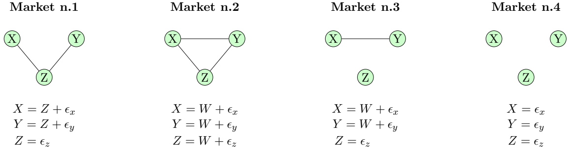
Figure 1: Toy example of graphs substructures in a financial market with three assets. Market n.1: the asset Z acts as common risk factor in the market driving the dependence and is a hub. Market n.2: the return of all three assets X , Y , and Z are driven by an unobservable risk factor W and the three assets form a clique. Market n.3: X and Y are driven by a common risk factor, not affecting the asset Z . Market n.4: the three assets are independent and the graph does not include any edge. Here \epsilon_z, \epsilon_x, \epsilon_y are white noises.
