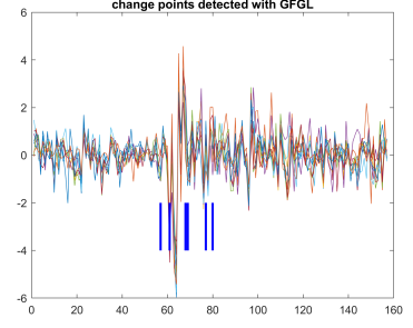
(c) The change points identified with \lambda_1 = 0.55 and \lambda_2 = 10 are \{57, 61, 68, 69, 77, 80\} .
