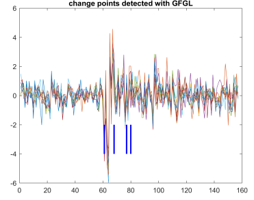
(f) The change points identified with \lambda_1 = 0.5 and \lambda_2 = 20 are \{61, 68, 77, 80\} .
