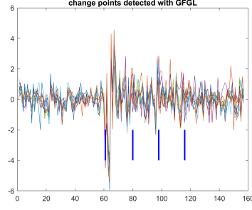
(b) The change points identified with \lambda_1 = 0.35 and \lambda_2 = 10 are \{61, 80, 98, 116\} .
