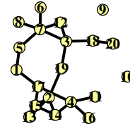
Figure B.1.3: Scenario 4: graph structure used as data generating mechanism for assessing model's performance.
