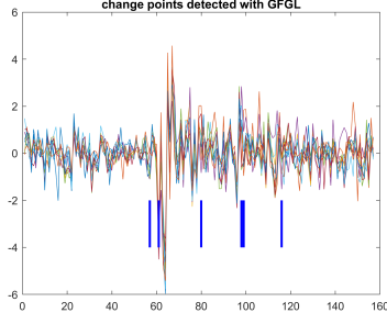
(a) The change points identified with \lambda_1 = 0.25 and \lambda_2 = 10 are \{57, 61, 80, 98, 99, 116\} .
