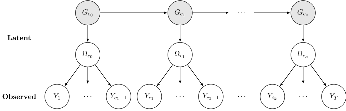
Figure 3: Graphical representation of the model conditionally on change points. Both graph and precision matrix are constant between change points. Observations ( Y_t ) are independent conditionally on the model parameters over time, while are iid between change points. Moreover, the precision matrices \{\Omega_{c_i}, i = 1, \dots, \kappa\} are conditionally independent given the sequence \{G_{c_i}, i = 1, \dots, \kappa\} .
