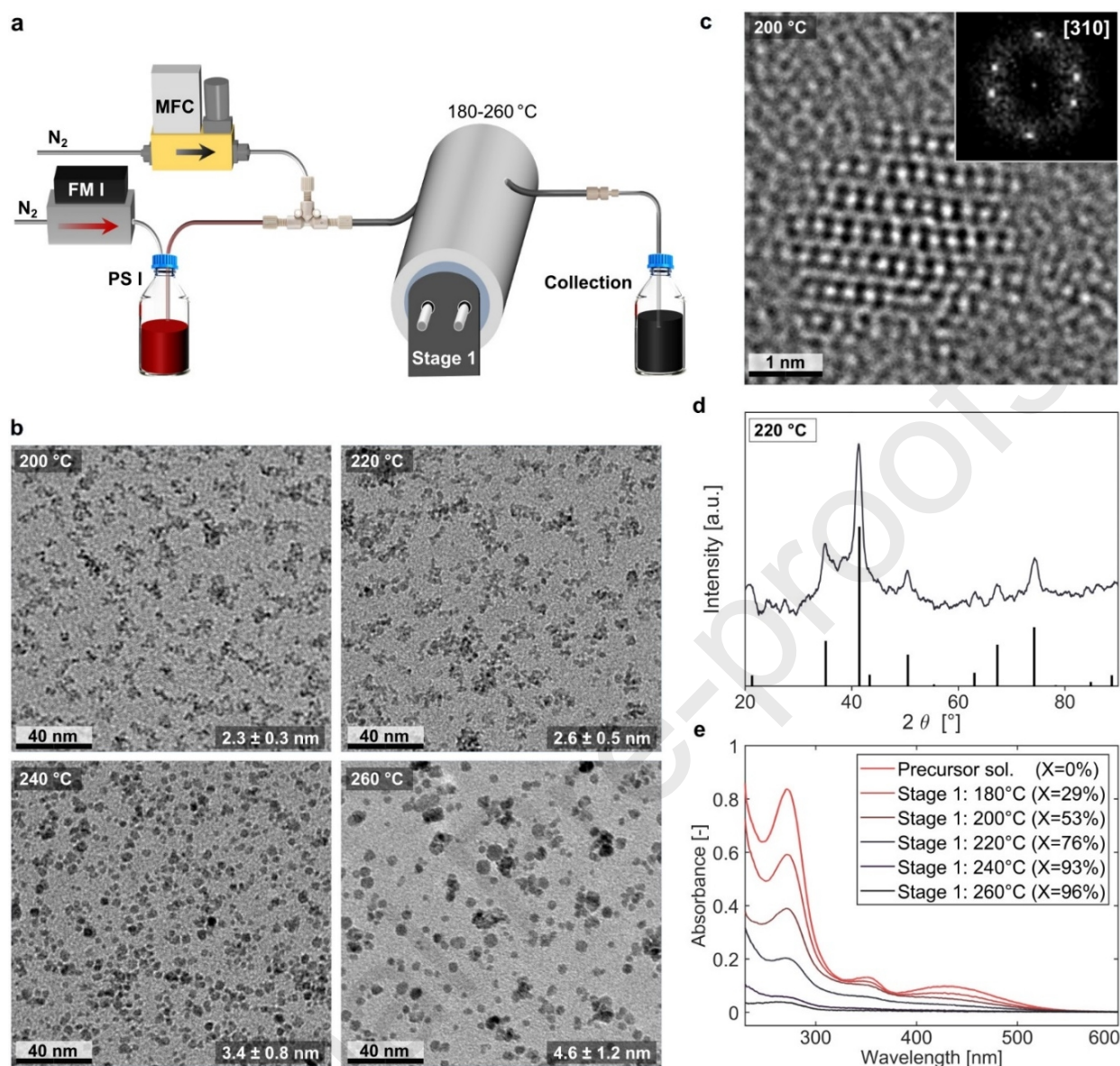
Figure 2: (a) Schematic of single-stage reactor set-up. (b) TEM images of IONPs synthesised via single stage (Stage 1) process, set between 200 °C and 260 °C. (c) HRTEM image of the ultra-small ( \leq 3 nm) IONPs synthesised at Stage 1 at 200 °C. The inset shows the fast Fourier transformation (FFT) indexed to a magnetite/maghemite [310] zone axis, taken from the particle. (d) XRD pattern of IONPs synthesised with Stage 1 at 220 °C. The bars at the bottom refer to the inverse spinel structure (magnetite: PDF ref. 03-065-3107). (e) UV-Vis spectra of precursor and IONP solutions diluted in IPA.
