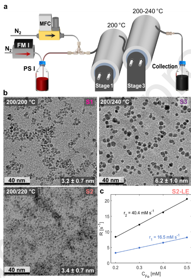
Figure 3: (a) Schematic of two-stage reactor set-up. (b) TEM images of IONPs synthesised via two-stage process with Stage 1 at 200 °C and Stage 3 at 200 °C (S1), 220 °C (S2) and 240 °C (S3). (c) The transversal (black line) and longitudinal (blue line) magnetic relaxation rates ( R ) vs. consecutively diluted iron concentrations ( C_{\text{Fe}} ) of ligand exchanged (LE) and dialysed aqueous IONP solution (S2) are used to determine the relaxivities r_2 and r_1 (i.e., the slope).
