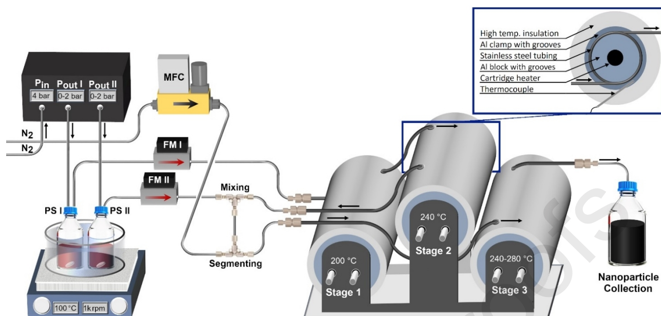
Figure 1: Schematic of the continuous thermal decomposition synthesis set-up. MFC: mass flow controller, FM: flowmeter, PS: precursor solution.
