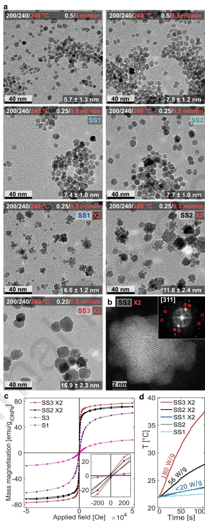
Figure 4: IONP synthesised via self-seeded three-stage process, with new precursor added before Stage 3. (a) TEM images of IONPs; the inset notation lists Stage 1/2/3 temperatures, flow rates PS I/PS II, and with X2 doubled PS II concentrations. (b) HRTEM and inserted FFT indexed to the [311] zone axis for sample SS2 X2; red circles are reflections
