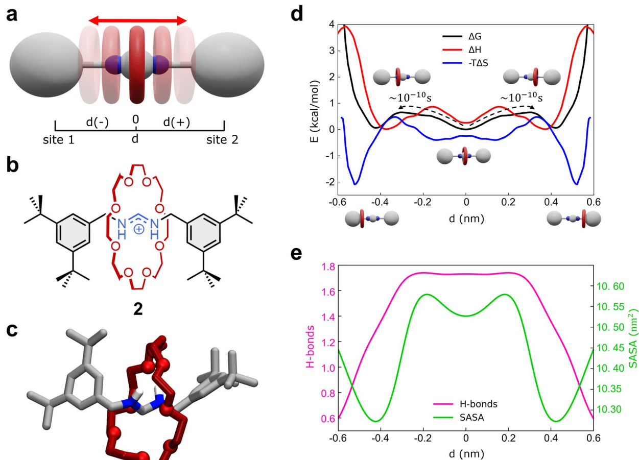
Fig. 3 Shuttling dynamics of the formamidinium [2]rotaxane (2). (a) Schematic representation of the mechanism of shuttling along the translational position d of the macrocycle, and (b) structural, chemical formula of the formamidinium [2]rotaxane (2). (c) AA molecular model of 2. Only the hydrogens of the recognition sites are displayed for clarity. (d) Free-energy (black), enthalpy (red) and entropy (blue) profiles associated with the system. The associated transition times are estimated via single-transition MD simulations. (e) Number of HBs between the crown and the thread (purple line) and SASA of the rotaxane (green line) as a function of d .
