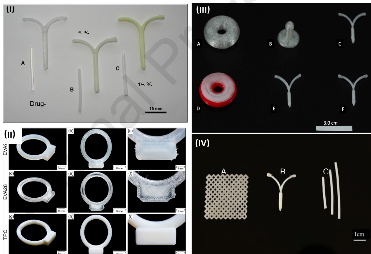
Fig. 7. (I): Images of filaments and 3D printed IUD using EVA 5: (A) drug-free, (B) and (C) 5% and 15 % indomethacin. Reproduced with permission from Genina et al., 2016[49], Elsevier, 2023, (II): Images of 3D printed implants using FDM technology with EVA and TPC showing visible difference in the quality of the printouts (Reproduced with permission from Koutsamanis et al., 2021[60], Elsevier, 2023, (III): Images of 3D printed constructs of passerines (A, B and D) and IUD (C, E and F) and (IV): Images of 3D printed estrogen mesh
