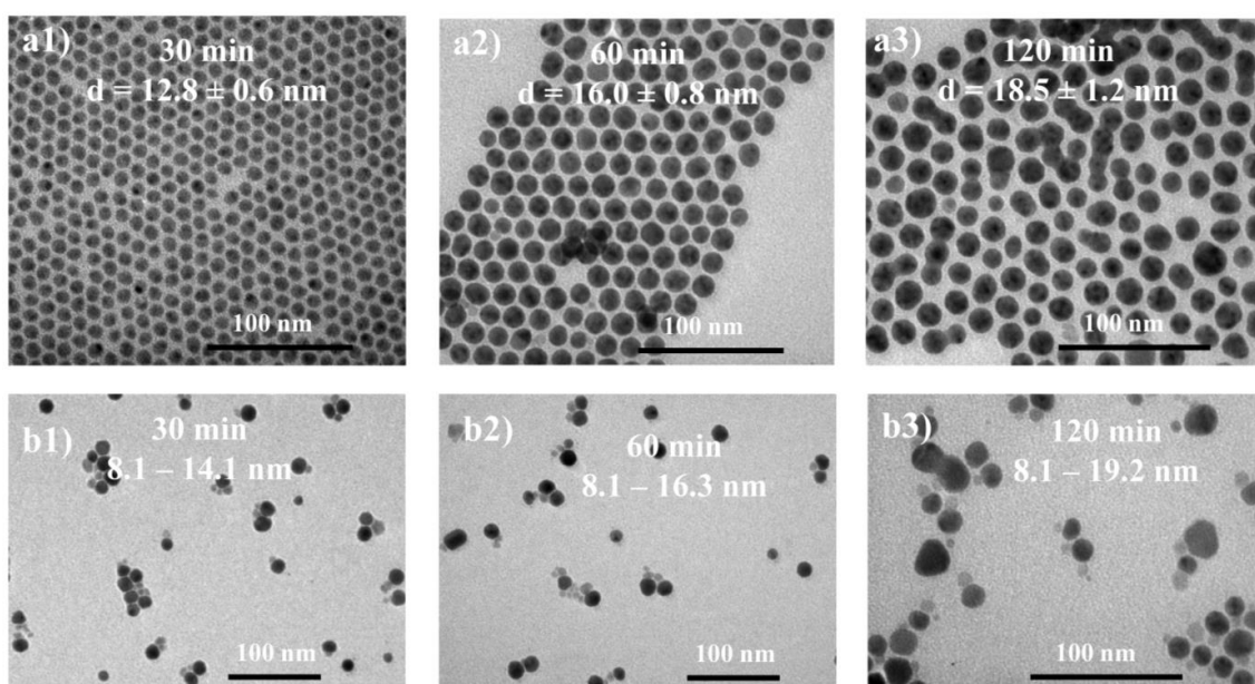
Fig. S4 TEM images of HNP synthesised with \text{Fe}_3\text{O}_4 seeds of 8.1 nm at different reaction times: (a1-a3) core-shell \text{Fe}_3\text{O}_4 @Ag HNPs and (b1-b3) dumbbell-like \text{Fe}_3\text{O}_4 -Ag HNPs.
