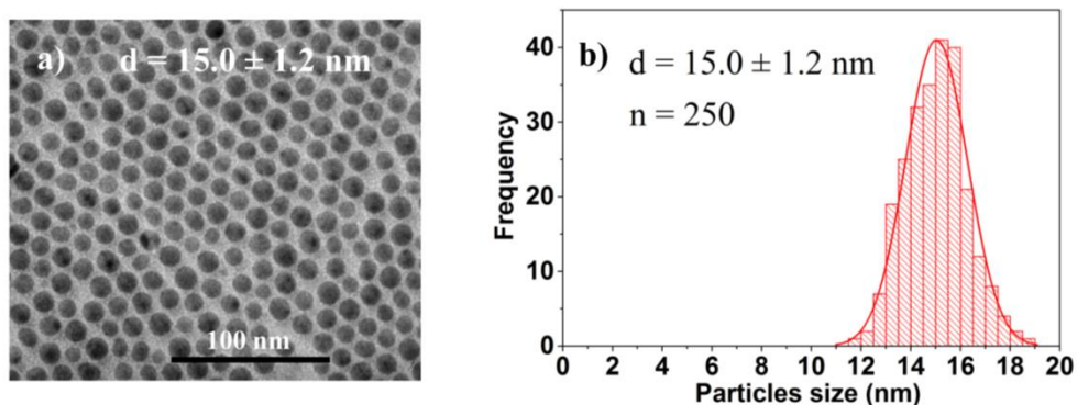
Fig. S3 TEM image and size distribution histogram of Ag nanoparticles synthesised under similar conditions but without \text{Fe}_3\text{O}_4 NPs at reaction time of 60 min.
