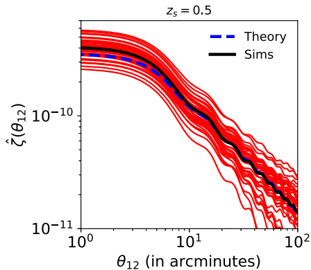
FIG. 1. The sq3PCF \zeta(\theta_{12}) defined in Eq. (4.6) for the convergence map \kappa for z_s = 0.5 is shown as a function of \theta_{12} . The dashed line corresponds to the theoretical prediction. The thin solid lines correspond to the estimates from individual simulated convergence maps computed using 192 nonlocal patches described in Sec. III. The thick solid line represents the ensemble average of estimates from all maps. A total of 40 maps were used.
