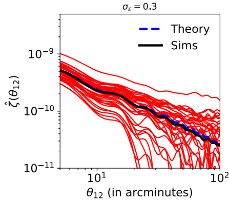
FIG. 6. Same as Fig. 1 but with an Euclid -like mask and noise included. We use a pseudo-Euclid mask which removes both the galactic and elliptic planes. The resulting fraction of sky coverage is f_{\text{sky}} = 0.35 (see Ref. [29] for more details). We also assumed Gaussian noise, with a noise power spectrum amplitude given by n_\ell = \sigma_\epsilon^2/\bar{N} . We have taken \bar{N} = 30 arcmin as expected for Euclid . We have also taken \sigma = 0.3 . The sources are placed at a redshift z_s = 1 .
