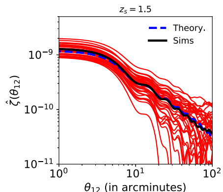
FIG. 3. Same as Fig. 1 but for z_s = 1.5 .
