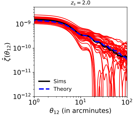
FIG. 4. Same as Fig. 1 but for z_s = 2.0 .
