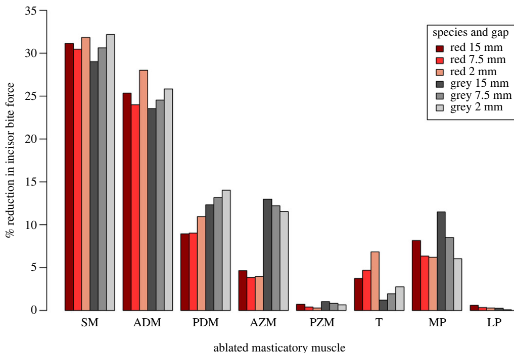
Figure 2. Percentage reduction in maximum incisor bite force for the red squirrel (red colours) and grey squirrel (grey colours) models with each pair of masticatory muscles set to zero activation. Darker shades represent wider gapes. ADM, anterior deep masseter; AZM, anterior zygomatic-mandibularis; LP, lateral pterygoid; MP, medial pterygoid; PDM, posterior deep masseter; PZM, posterior zygomatic-mandibularis; SM, superficial masseter; T, temporalis.
