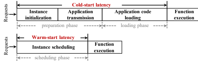
Fig. 1. The latency breakdown after requests come in cold and warm starts.
