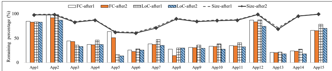
Fig. 4. The change of statistical values (the optimized application as a percentage of the original application).
