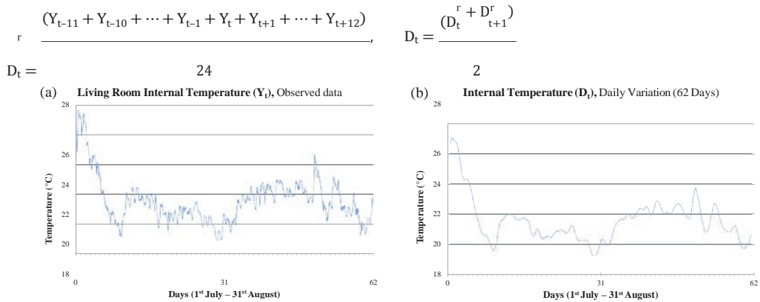
Figure 3. (a) temperature profiles of observed data; (b) temperature profiles of daily variation.
