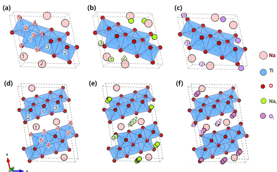
Figure 2. Crystal structures of conventional (a–c) \text{Na}_2\text{Ti}_3\text{O}_7 ( P2_1/m ) and (d–f) \text{Na}_2\text{Ti}_6\text{O}_{13} ( C2/m ), showing the symmetry unique defect sites used in defect calculations.
