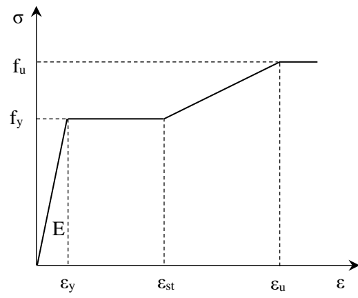
Fig. 7 Stress–strain curve of steel beam (reproduced from [21])
