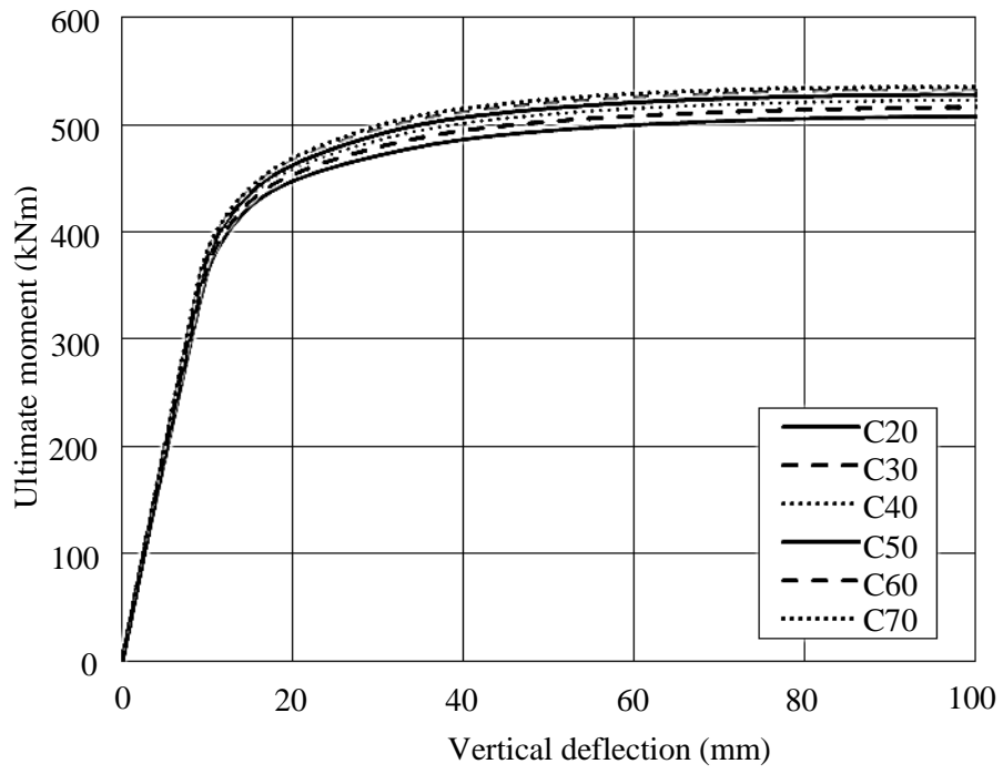
Fig. 19 Influence of concrete strength on the behaviour of CFTFGs
