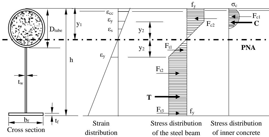
Fig. 11 Distributions of strain and stress for Case 2, where the PNA is in the tubular flange section ( y_1 < D_{tube} ).
