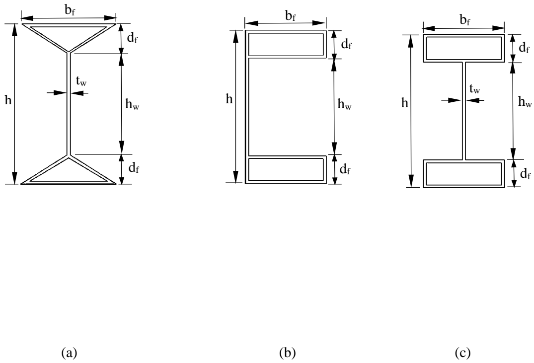
Fig. 1. Hollow flange girders including (a) triangular hollow flange beam, (b) LiteSteel beam and (c) rectangular hollow tubular flange plate girder.
