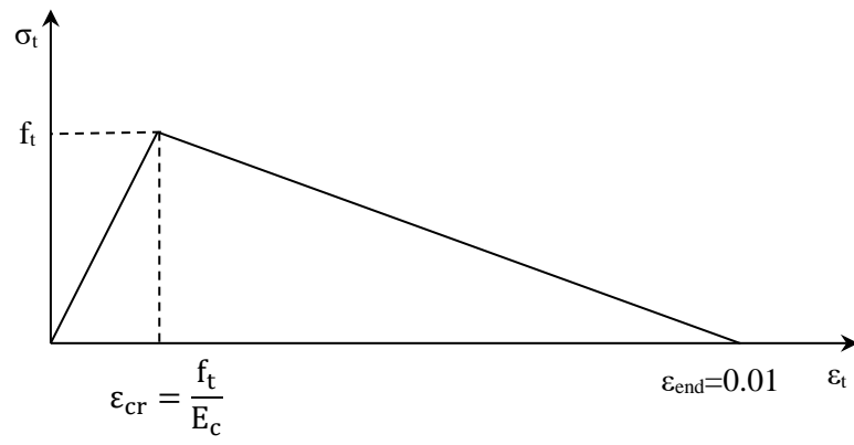
Fig. 6 Tensile stress-strain curve for concrete
