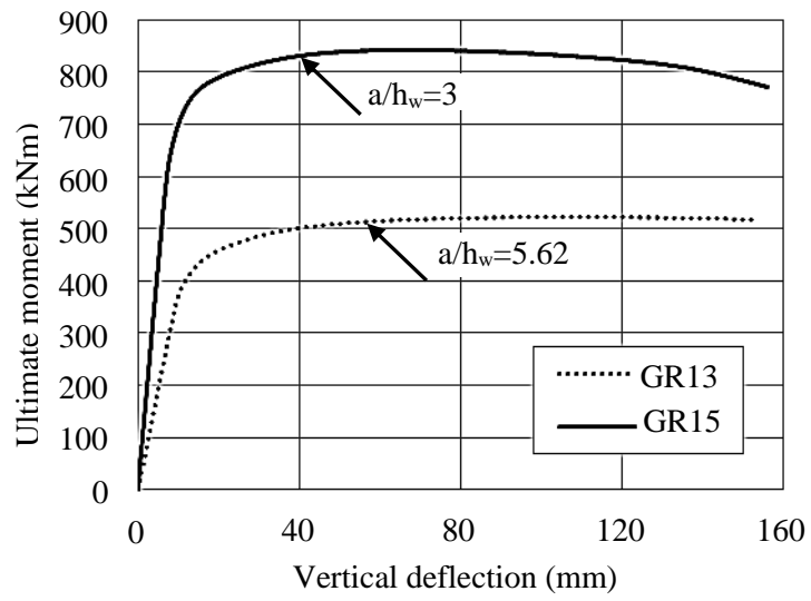
Fig. 16 Ultimate moment versus deflection for GR13 and GR15 with difference web panel aspect ratios
