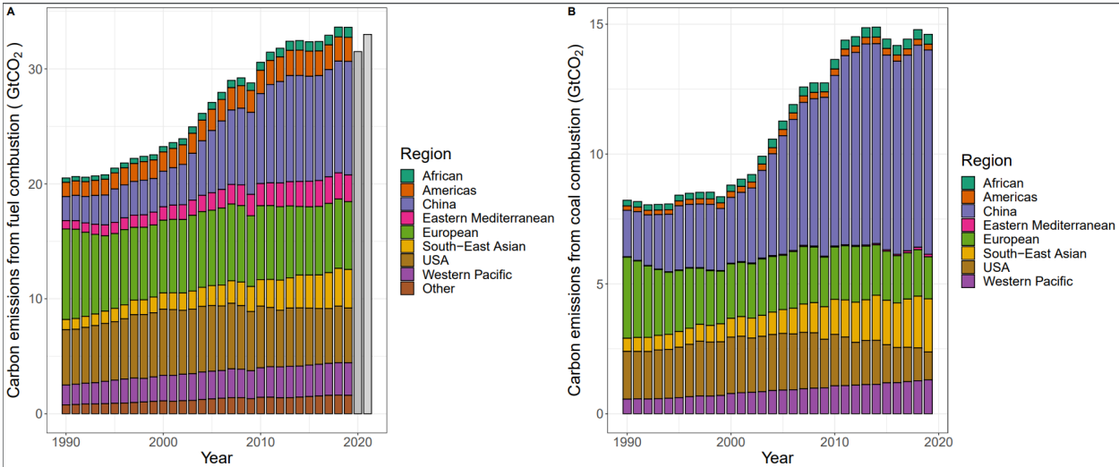
Figure 7: Greenhouse gas emissions from the global energy system. Panel A: Global CO 2 emissions from fossil fuel usage. Preliminary and modelled values shown for years 2020 and 2021 respectively. Panel B: Global CO 2 emissions from the use of coal
