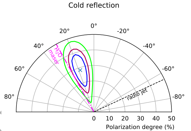
Figure 5. Contour plot of the polarization degree and angle for the cold reflector. The blue, red and green lines correspond to the 68, 90 and 99 per cent confidence levels, respectively. The black dashed line marks the direction of the radio jet, while the magenta dash-dotted line marks the direction of the inner \text{H}_2\text{O} maser disc.
