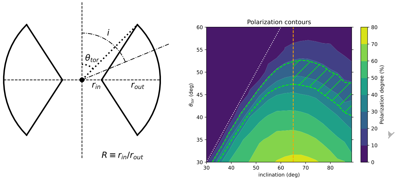
Figure 6. Left panel: Sketch of the torus geometry assumed for polarimetric modelling. The torus opening angle \theta_{\text{tor}} and the observer inclination i are both measured from the symmetry axis. Right panel: Contour plots of the constant polarization degree calculated for scattering off a torus, on the \theta_{\text{tor}} - i plane. The white dotted line corresponds to the equality \theta_{\text{tor}} = i ; the condition for the obscuration of the central source is \theta_{\text{tor}} < i . The green dashed curves enclose the 68 per cent confidence level region on the measured polarization for the cold reflector in the Circinus galaxy. The orange dashed line marks the inclination of the host galaxy, likely a lower limit to the torus inclination (as discussed in the text). The green hatches mark the region of the parameter space consistent with all the observational constraints.
