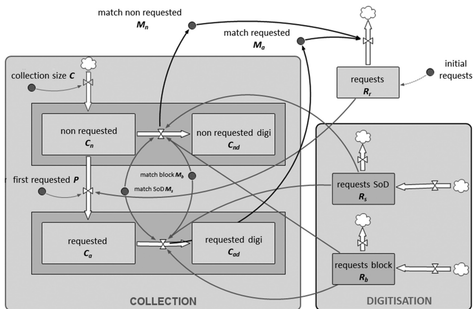
Figure 5. Proposed system dynamics model to simulate the relationship between the level of demand in the reading room and the digitisation of the physical collections.
