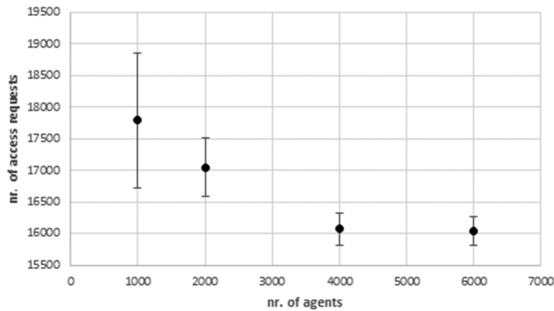
Figure 7. Comparison of the ABM output (number of access requests in the reading room at the end of the run, R_r ) depending on the number of agents. Error bars indicate the standard deviation.
