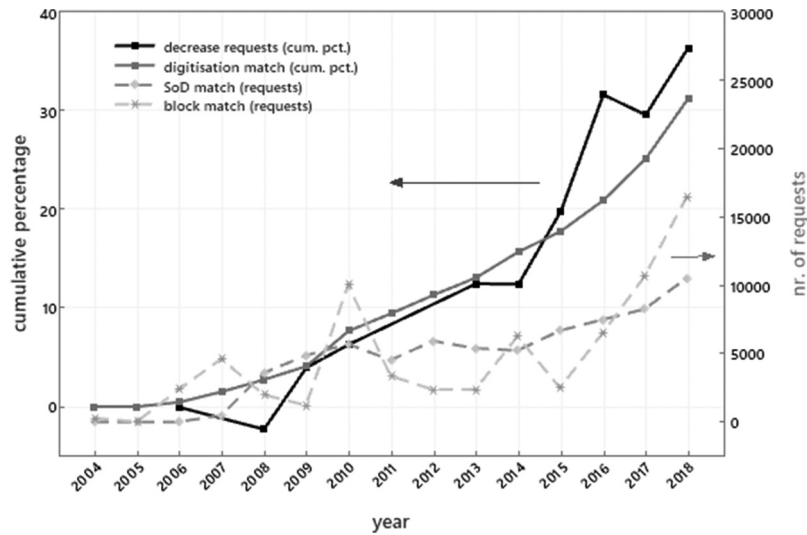
Figure 4. Cumulative percentage of the decrease in requests at the Amsterdam city archives (2007, 2011 and 2012 not included) and “digitisation match” since 2006. The dashed lines show the number of access requests digitised within the two digitisation programmes, SoD and the digitisation of block of archives.
