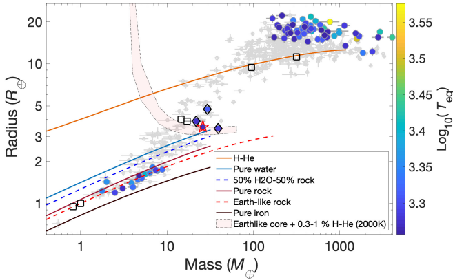
Fig. 10: Mass-radius diagram of all known planets up to 13 M_J with 30 % and 10 % uncertainties or lower in mass and radius, respectively. Planets with T_{eq} \geq 1800 K are colour-coded with T_{eq} , and the rest are plotted in light grey. In total, there are four planets (including TOI-2196 b) with radii between 3 and 5 R_{\oplus} in this diagram that are identified as hot Neptune desert planets (cf. Fig. 9). TOI-2196 b is marked with a red star symbol and the three additional planets with black diamonds. Solar system planets are marked with brown squares. Interior models from Zeng et al. (2019) are plotted as listed in the legend. The 100 % water line is for a planet with condensed water phases.
