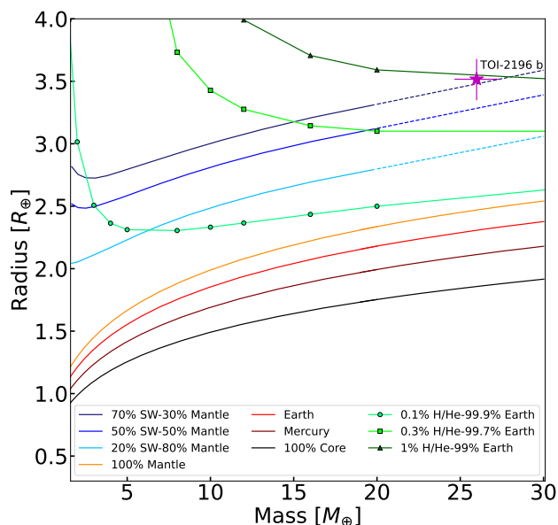
Fig. 13: Position of TOI-2196 b in the mass-radius diagram. We also show mass-radius relationships for dry planets with different core mass fractions (Brugger et al. 2016; Brugger et al. 2017), water planets with varying supercritical water (SW) contents (Mousis et al. 2020; Acuña et al. 2021) and Earth-like cores with different H/He mass fractions (Zeng et al. 2019). We assume equilibrium temperatures of 1200 K and 2000 K for water planets and rocky planets with H/He atmospheres, respectively. Dashed lines indicate an extrapolation of the SW relations beyond their valid mass ranges. The lines for Earth, Mercury, and 100 % core are lines of constant composition of respective type of planet.
