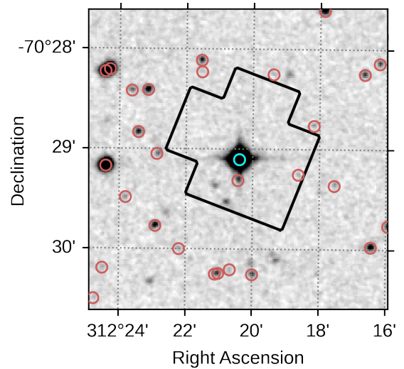
Fig. 1: 3' × 3' DSS2 image (red filter) centered on TOI-2196 (cyan circle). The SPOC photometric aperture of sector 27 is outlined in black while Gaia DR2 sources within 2' from the target are marked by the red circles.
