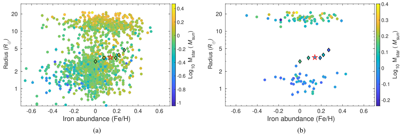
Fig. 12: Planet radius vs. iron abundance diagram of the same planets as in Fig. 9: a) colour-coded with stellar mass b) Same but only plotting planets with T_{\text{eq}} \geq 1800 K, which corresponds to P_{\text{orb}} \lesssim 1.3 d for a sun-like star assuming zero Bond albedo and a heat redistribution factor of unity, or P_{\text{orb}} \lesssim 0.43 d for a K5 V star.
