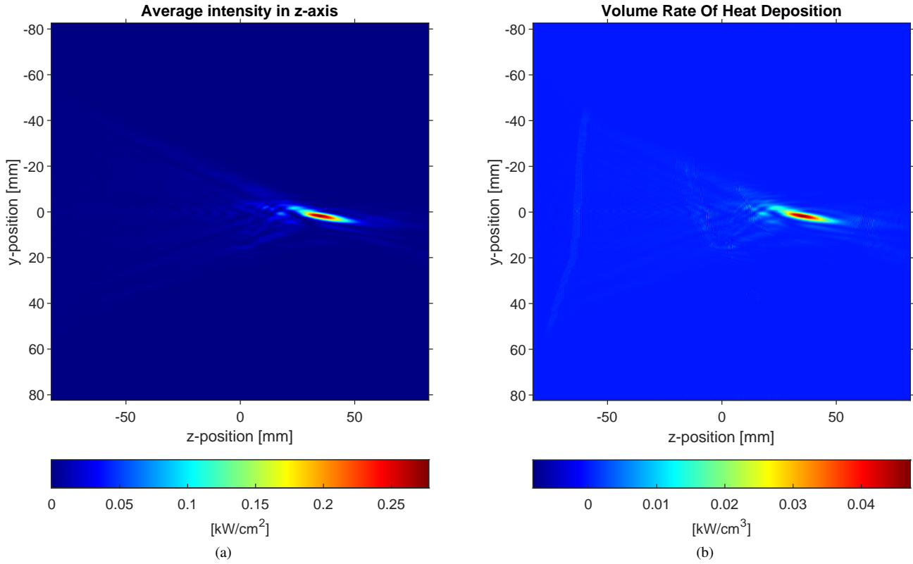
Fig. 3. Visualization of average intensity in z-axis (a) and volume rate of heat deposition (b) without the compression.
