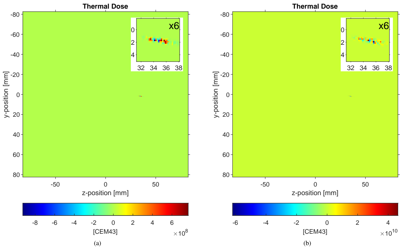
Fig. 7. Visualization of the thermal dose errors. The compression error is on the left (a), the 40-bit compression error on the right (b).
