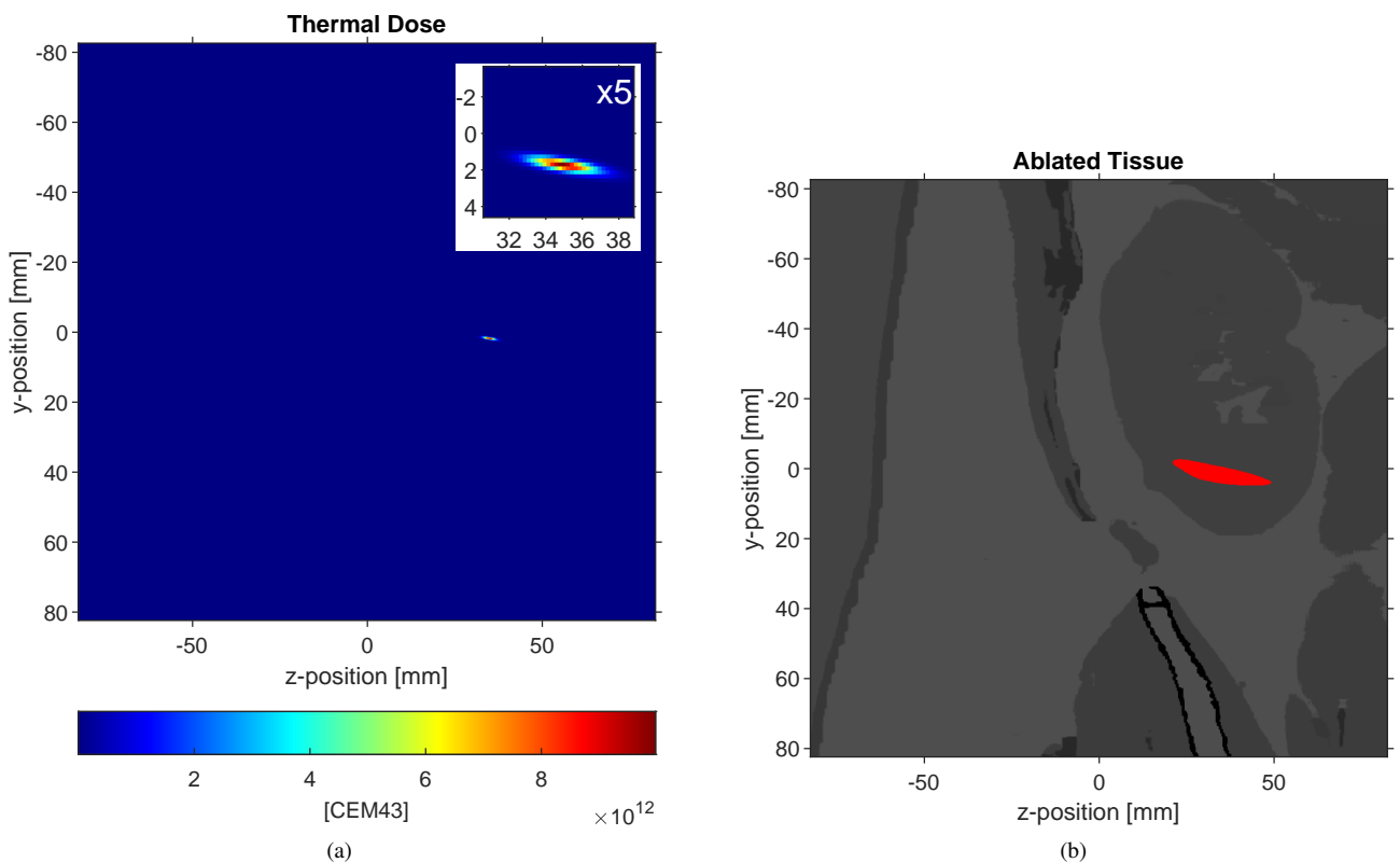
Fig. 6. Visualization of thermal dose (a) and ablated tissue (b) without use of the compression.
