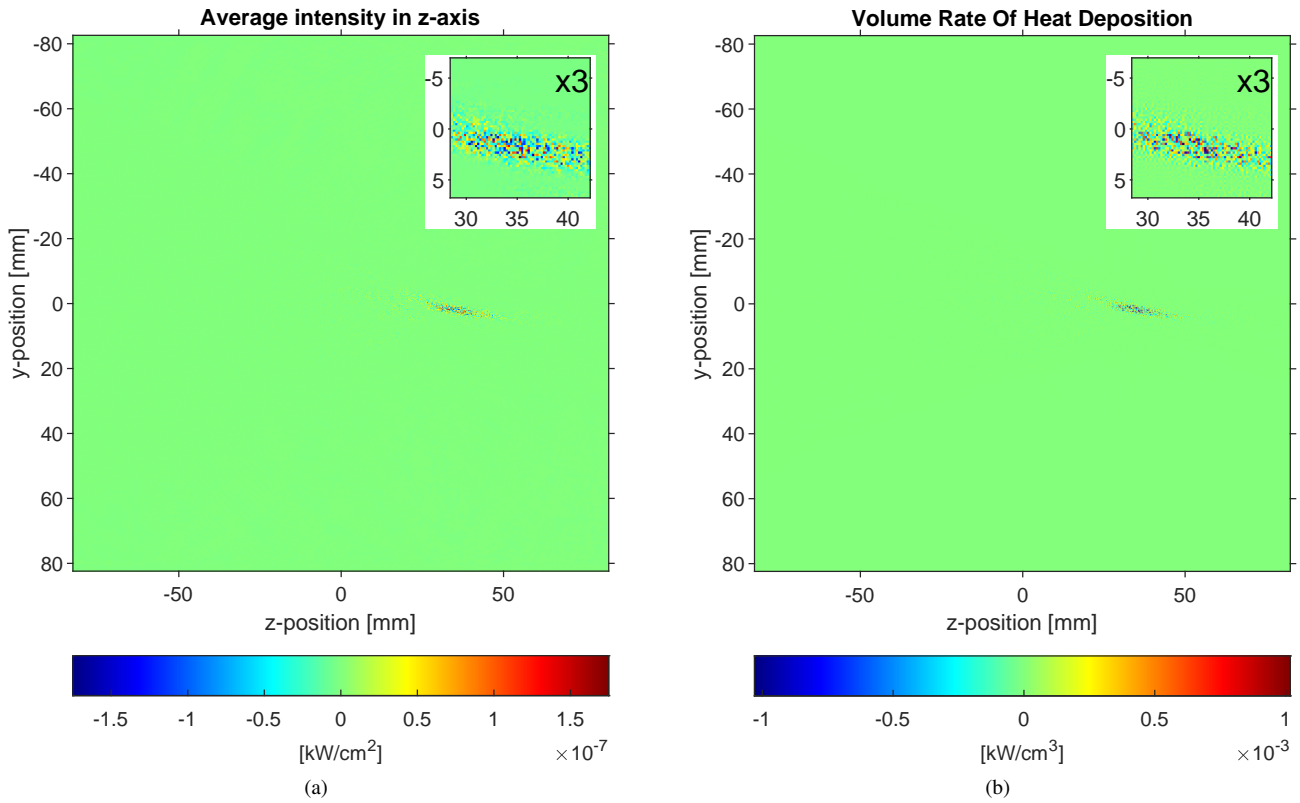
Fig. 5. Visualization of average intensity error in z-axis (a) and volume rate of heat deposition (b) with the 40-bit compression.
