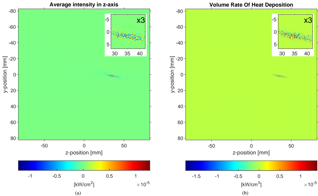
Fig. 4. Visualization of average intensity error in z-axis (a) and volume rate of heat deposition (b) with the compression.
