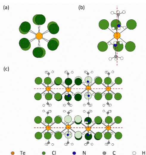
Fig. 2 Schematic of MA 2 TeCl 6 (III) showing (a) the rotational twist about the c -axis of the [Te(1)Cl 6 ] 2- anions from one octahedral layer to the next layer; (b) the minor tilting of the C–N axis of the MA + cation relative to the c -axis (shown as dashed red line); and (c) the slight positional offset of the octahedra in each layer, where red dashed lines represent ab planes at c = 0 and c = \frac{1}{2} . The green colour shades are used to distinguish the Cl atoms belonging to different octahedra.
