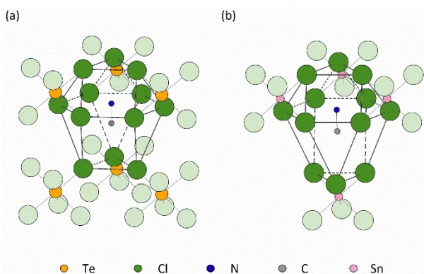
Fig. 7 Schematic diagram of the MA + cations located in (a) a cavity coordinated by 6 [TeCl 6 ] 2- anions in MA 2 TeCl 6 and (b) the cavity formed by only 4 [SnCl 6 ] 2- anions in MA 2 SnCl 6 . For clarity, hydrogen atoms are not shown.
