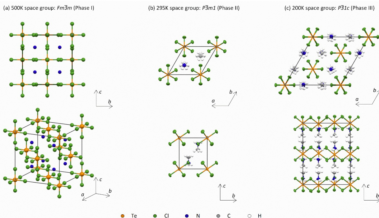
Fig. 1 The crystal structure of MA 2 TeCl 6 in (a) phase I at 500 K seen down the a -axis shown (upper) and obliquely (lower) in which a single N atom represents the whole MA + cation due to the dynamical free rotation; (b) phase II at 295 K seen along the c -axis (upper) and down the a -axis (lower); and (c) phase III at 200 K seen along the c -axis (upper) and down the a -axis (lower).
