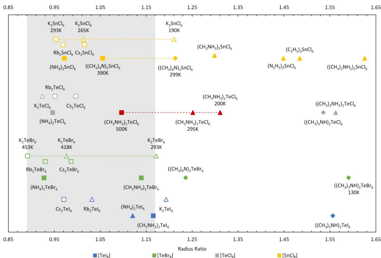
Fig. 9 Radius ratio for \text{A}_2\text{TeX}_6 and \text{A}_2\text{SnCl}_6 compounds calculated from the shortest d_{\text{A-X}} values. The \text{MA}_2\text{TeCl}_6 phases determined in this work are highlighted in red. Fm\bar{3}m cubic structures are found in the range 0.89 - 1.17 as picked out in grey. (Square, diamond, and triangle symbols represent the Fm\bar{3}m cubic structure, other cubic structures, and non-cubic structures respectively; solid symbols represent organic cation structures and hollow symbols represent inorganic ones.)
