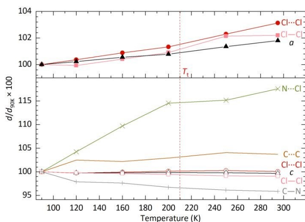
Fig. 8 Percentage interatomic distance changes, d/d_{90K} , as projected in a and c for a variety of atoms in MA 2 TeCl 6 as a function of temperature relative to the structure at 90 K; the values are derived from SXD. Although there is a significant percentage increase in N...Cl with respect to c , in absolute terms, this contributes only a small to expansion in c . The error bar is smaller than the symbol; all error values can be found in Table S2 and Table S3 † .
