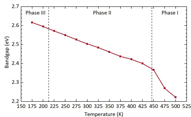
Fig. 5 Optical bandgap of \text{MA}_2\text{TeCl}_6 calculated as a function of temperature from the Tauc plot shown in Fig. S8†.
