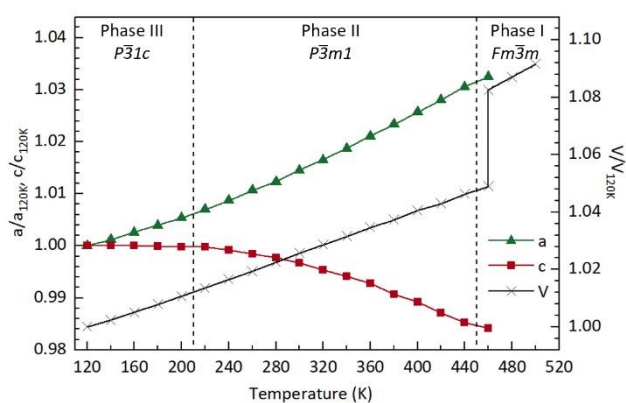
Fig. 4 Plot showing the variation (compared with T = 120 K) in lattice parameter and volume as a function of temperature obtained from fits to the data using GSAS II 10 . Values are given in Table S1†. Lines joining the data points are a guide to the eye.
