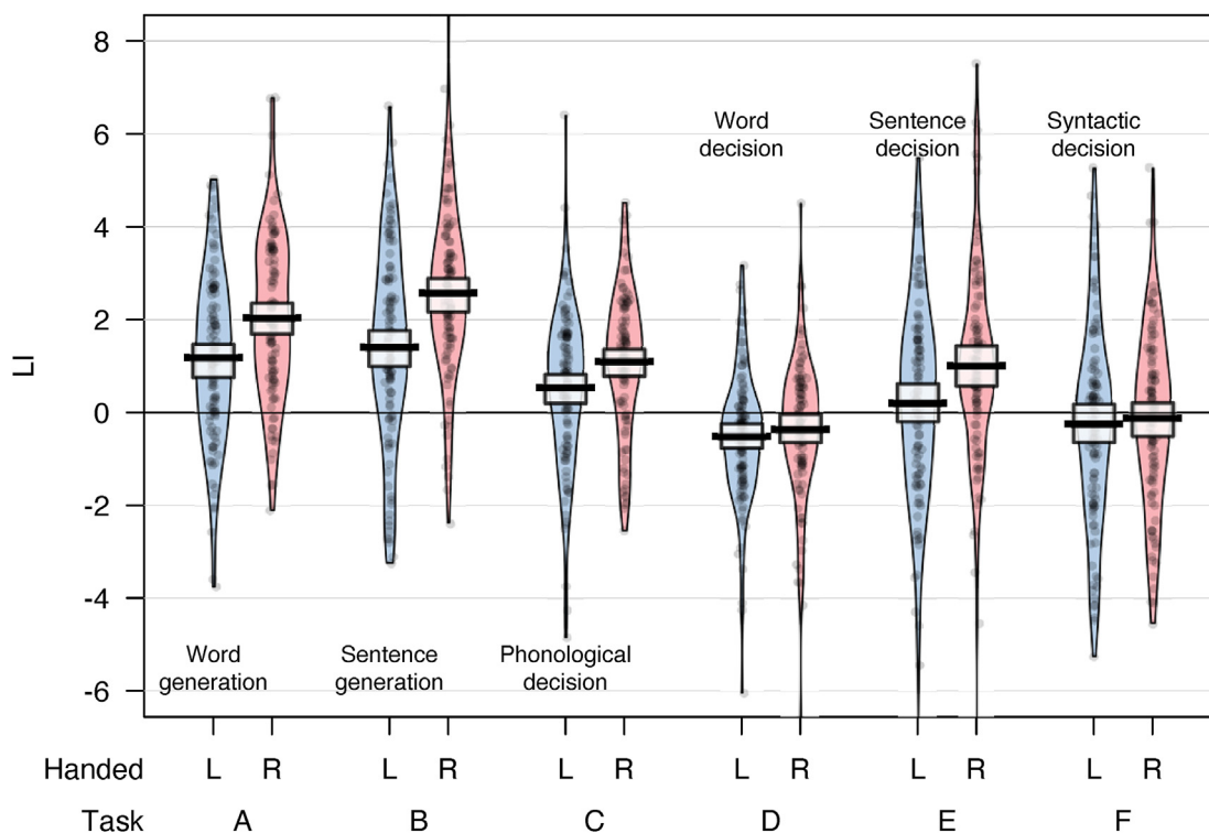
Fig. 7 – Distributions of fTCD LIs on six tasks for 104 left-handers and 91 right-handers.
