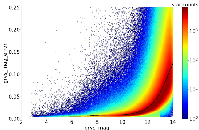
Fig. 13. Internal precision: grvs_mag_error plotted against grvs_mag . The black line shows the median grvs_mag_error in bins of \Delta(\text{grvs\_mag}) = 0.1 mag. This indicates a median grvs_mag_error around 0.006 mag over the range 4 \lesssim \text{grvs\_mag} \lesssim 6.5 mag, increasing to \sim 0.025 at grvs_mag \sim 12 mag, and \sim 0.125 at grvs_mag \sim 14 mag.
