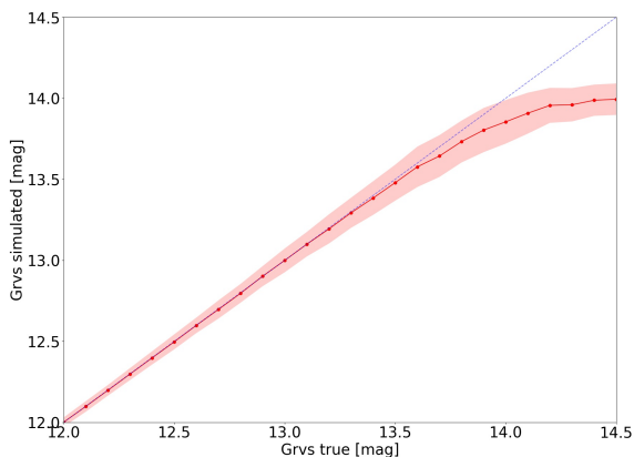
Fig. 6. grvs\_mag computed following the procedure outlined in Sect. 4.2, G_{\text{RVS}}^{\text{simu}} , plotted against true magnitude, G_{\text{RVS}}^{\text{true}} , for the simulations described in Sect. 6. The red line shows the median relation from 1000 realisations, and the shaded area the associated error. The dashed blue line shows the identity relation. The estimated magnitude becomes systematically brighter than the true one for G_{\text{RVS}}^{\text{true}} \gtrsim 13.3 . The limiting magnitude of the stars processed for DR3 corresponds to G_{\text{RVS}}^{\text{true}} = 14 .
