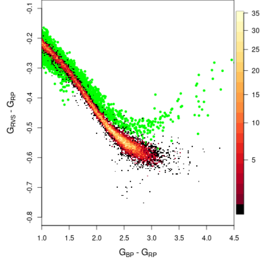
Fig. 19. grvs\_mag - G_{RP} versus G_{BP} - G_{RP} colour–colour diagram for cool stars in DR3. Low-extinction giants are represented with green dots, and nearby cool dwarfs with a red-coloured density plot.
