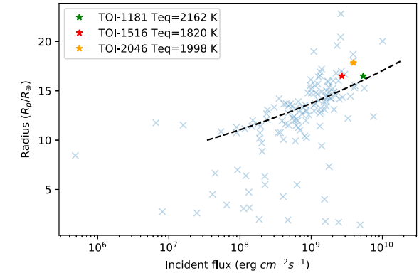
Figure 13. Radius versus incident flux for the three hot Jupiters from this paper including their equilibrium temperatures. Other known planets are represented by blue crosses. The dashed line represents the empirical relation from Weiss et al. (2013) for Jupiter-mass planets (equation 2).
