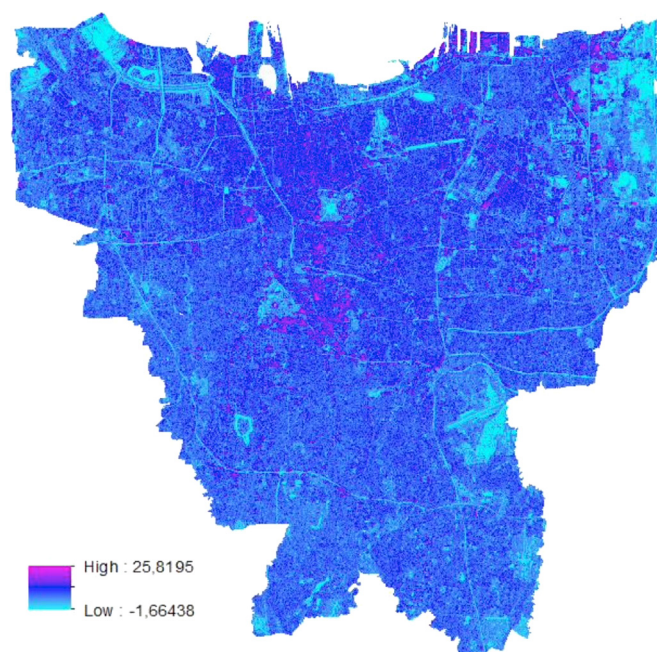
Fig. 2. Sentinel-1 (mean) Jan 2020.
