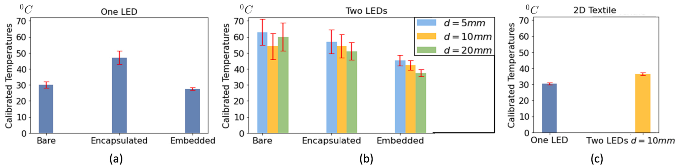
Fig. 12. Bar charts of the linear-interpolated and calibrated temperatures for one LED in its three different states; bare, encapsulated and embedded n (a); for two LEDs with different distances (b); and for 2D knitted garments for one and two LEDs embedded inside the yarn (c).
