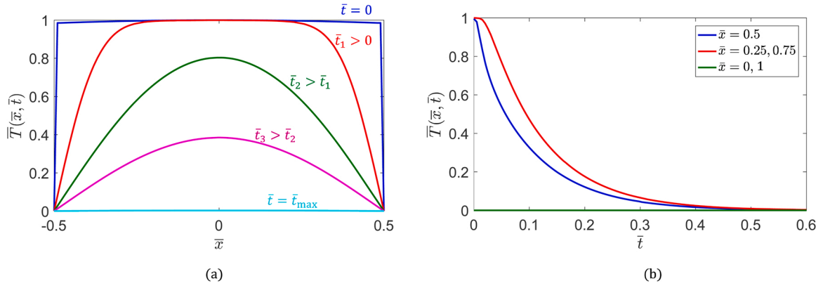
Fig. 2. The time-dependent temperature distribution \bar{T}(\bar{x}, \bar{t}) along one LED with a length L . (internal temperature distribution); (a) shows \bar{T}(\bar{x}, \bar{t}) as a function of the spatial variable \bar{x} for different time steps and (b) illustrates the temperature distribution behaviour as a function of time for different LED positions: \bar{x} = 0.5 (blue line), \bar{x} = 0.25, 0.75 (red line) and \bar{x} = 0, L (the green line). Here we have used: A = 1, \mu = 0 and \sigma = 4 and \bar{t}_{\max} = 0.6 . (For interpretation of the references to colour in this figure, the reader is referred to the web version of this article.)
