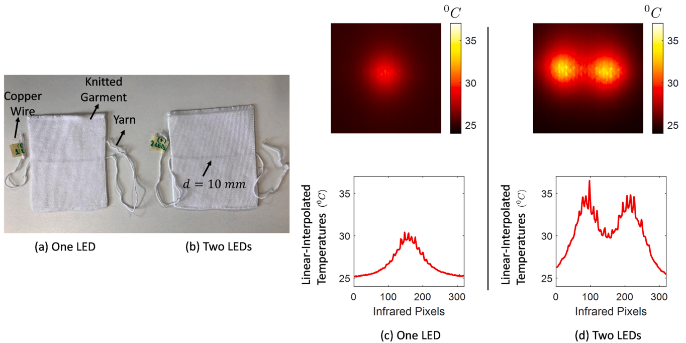
Fig. 11. 2D knitted garments with one LED in (a) and two LEDs in (b) with a distance d = 10\text{ mm} between both of them. 2D MATLAB generated images of the 2D knitted garments with the corresponding linear-interpolated thermal distribution plots are in (c) and (d). All temperatures are in ^{\circ}\text{C} .
