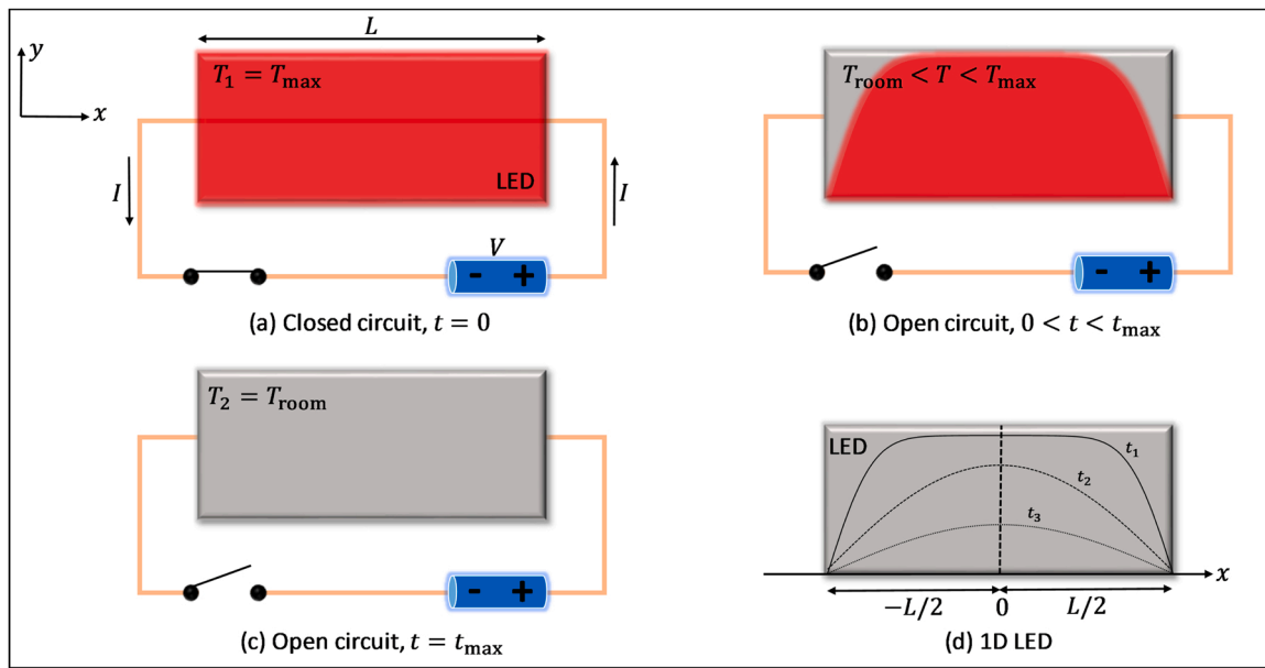
Fig. 1. Simplified schematics illustrating the thermal distribution within the LED at t = 0 in (a) when the electronic circuit is closed, at 0 < t < t_{\max} in (b) and at t = t_{\max} in (c) when the circuit is open. (d) is the 1D LED along x axis with the thermal distributions at times t_1 < t_2 < t_3 are presented along the LED.
