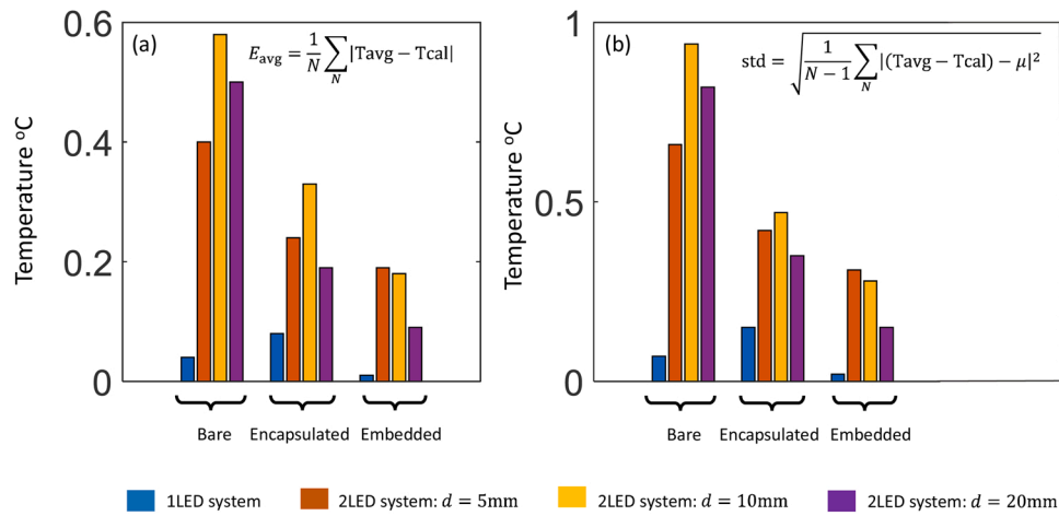
Fig. 13. Error analysis between the experimental and averaged smoothed data for all textile stages in both systems: one-LED and two-LED. (a) the average error, E_{avg} ; and (b) the standard deviation, std .
