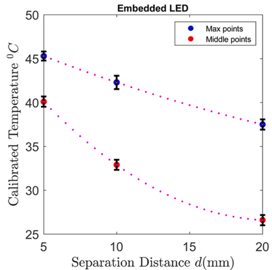
Fig. 16. The behaviour of the max (blue circles) and middle (red circles) points of Two-LED systems' thermal distributions as a function of separation distance between the two LEDs, d(\text{mm}) for the embedded yarn. (For interpretation of the references to colour in this figure, the reader is referred to the web version of this article.)
