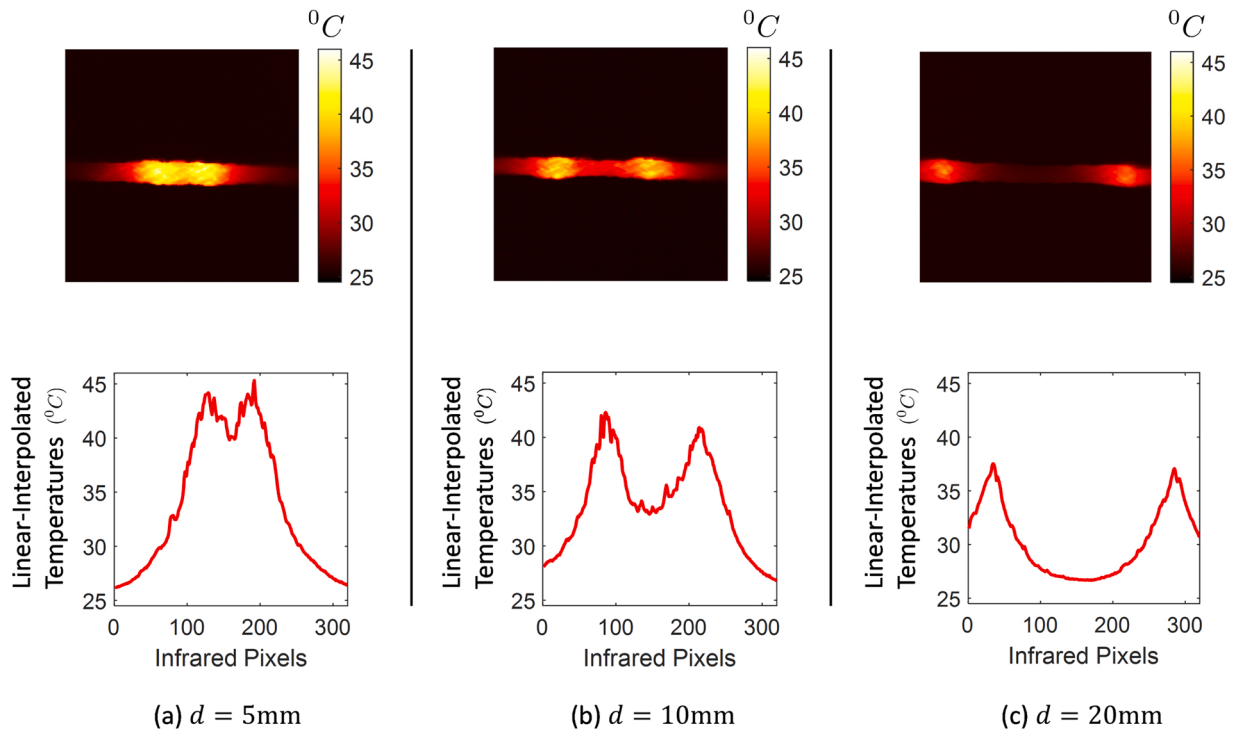
Fig. 10. Yarn embedded LEDs as (described in Section 3.2). Linear-interpolated 2D images created by MATLAB for two embedded LEDs and their corresponding thermal distribution plots; with the separation between both LEDs is d = 5\text{mm} in (a), d = 10\text{mm} in (b) and d = 20\text{mm} in (c). All temperatures are in ^{\circ}\text{C} .
