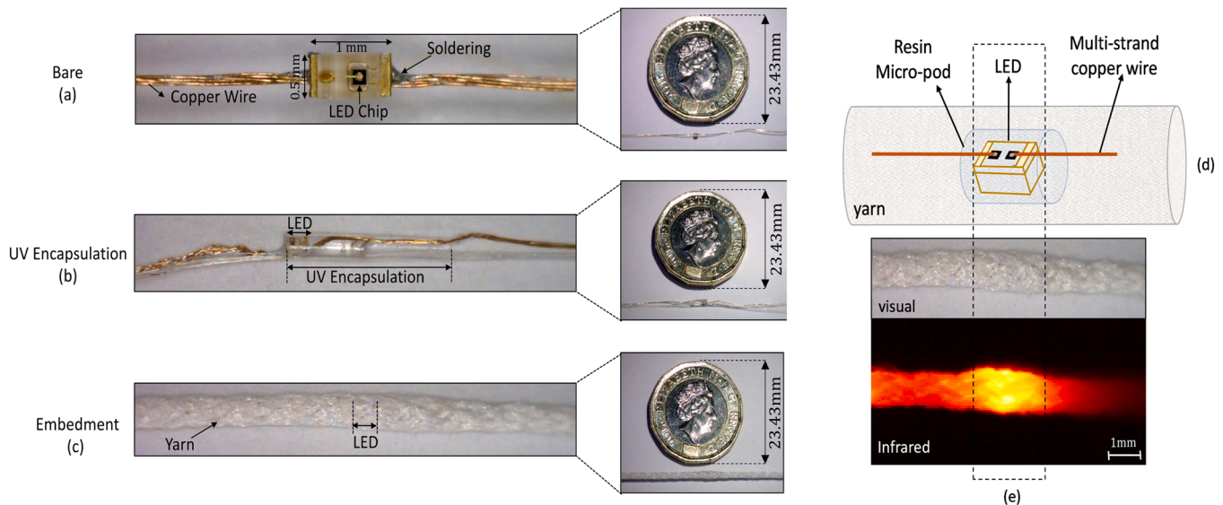
Fig. 6. Three basic states of LED followed in smart textiles technology. (a) is the bare LED and its dimensions, (b) the encapsulated LED and (c) the embedded LED inside the yarn, (d) a sketch that clarifies the structure of the final textile, and (e) shows the visual and infrared version of the final yarn.
