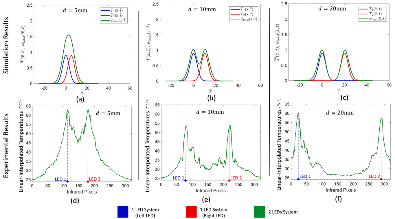
Fig. 15. The relationship between the separation distance between the two bare LEDs and the overall system temperature. Sub-figures (a), (b) and (c) show the mathematical simulation; while sub-figures (d), (e) and (f) show the experimental results. The green solid line represents the two-LED system and the blue and red lines represent the one-LED system. (For interpretation of the references to colour in this figure, the reader is referred to the web version of this article.)
