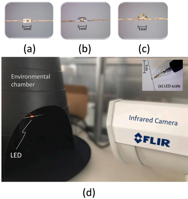
Fig. 5. Illustration of a bare LED used in our project where (a) shows the front, (b) the back and (c) the side views of the LED. The pictures were taken using a digital microscope: Dino-Lite AM-311S; the experimental work setup (d), the scale of LED in comparison to a standard ballpoint pen (biro) (e).
