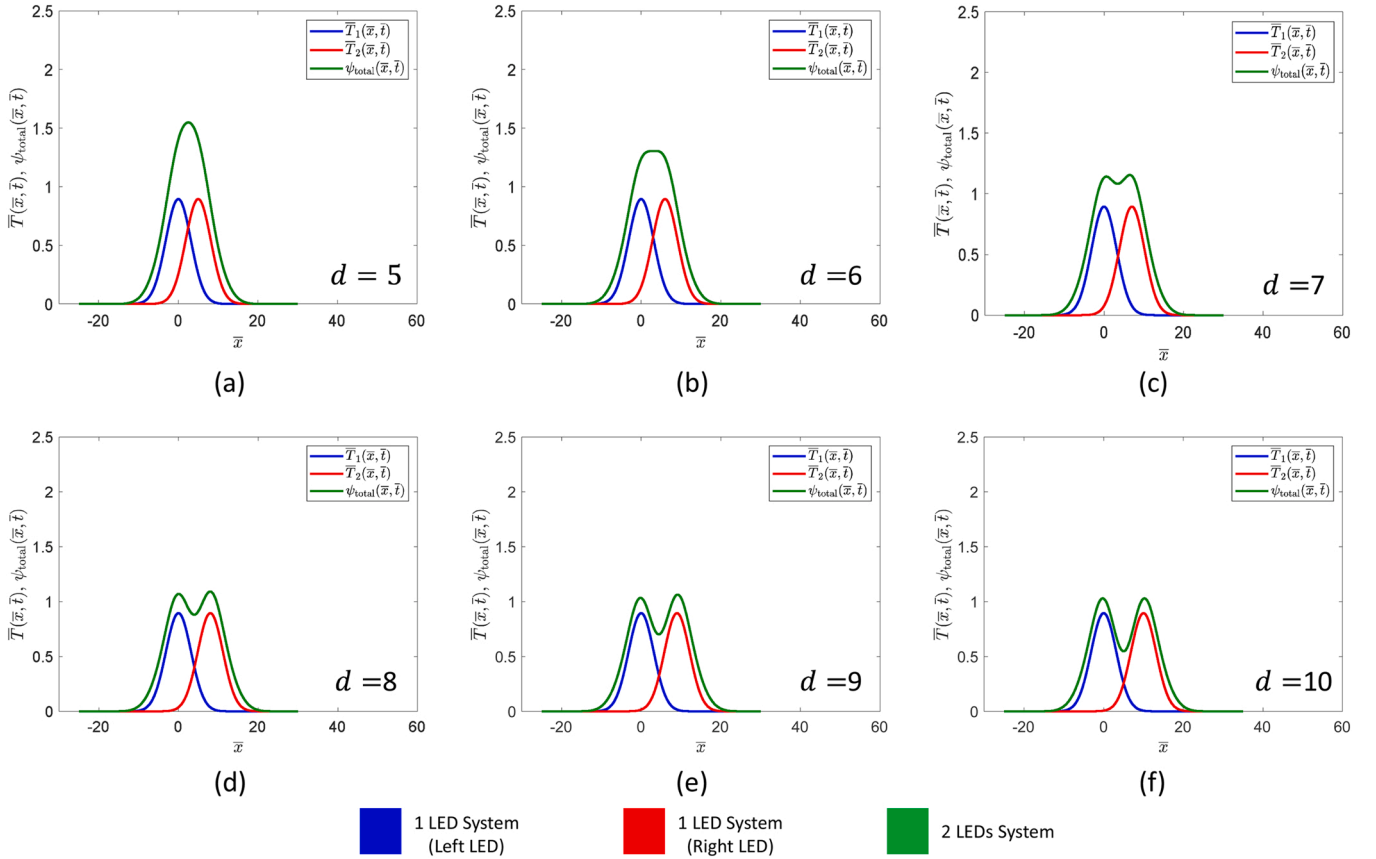
Fig. 4. The total thermal distribution of a two-LED system with mutual effect for different separation values d at \bar{t} = \bar{t}_{\max}/2 . The blue line represents the left LED, i.e., \bar{T}_1(\bar{x}, \bar{t}) , the red line represents the right one, i.e., \bar{T}_2(\bar{x}, \bar{t}) , and the green line refers to Eq. 11 where the total thermal distribution \psi_{\text{Total}}(\bar{x}, \bar{t}) is the sum of the modified solutions for each LED. Here we have used: for the corrected Gaussian function, \gamma_1 = -5 , \gamma_2 = 10 (a), 11 (b), 12 (c), 13 (d), 14 (e), 15 (f), s_{1,2} = 3 , h_{1,2} = \frac{1}{s_{1,2}\sqrt{2\pi}} = 0.13 , and for the initial source solutions A_{1,2} = 1 , \mu_1 = 0 , \mu_2 = 5 (a), 6 (b), 7 (c), 8 (d), 9 (e), 10 (f), \sigma_{1,2} = 4 and \bar{t}_{\max} = 2 . (For interpretation of the references to colour in this figure, the reader is referred to the web version of this article.)
