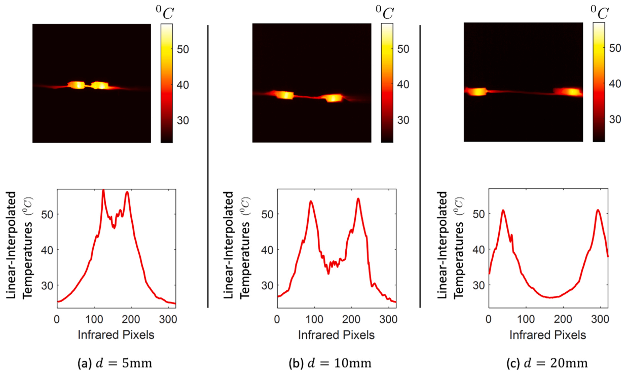
Fig. 9. Encapsulated LEDs. Linear-interpolated 2D images created by MATLAB for two encapsulated LEDs and their corresponding thermal distribution plots; with separation distance ( d ) between both LEDs of d = 5\text{mm} in (a), d = 10\text{mm} in (b) and d = 20\text{mm} in (c).
