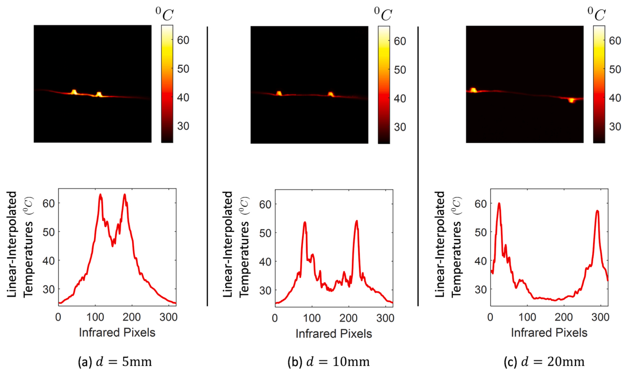
Fig. 8. Bare LEDs. Linear-interpolated 2D images created by MATLAB for two bare LEDs and their corresponding thermal distribution plots; with separation distance ( d ) between both LEDs of d = 5\text{mm} in (a), d = 10\text{mm} in (b) and d = 20\text{mm} in (c).
