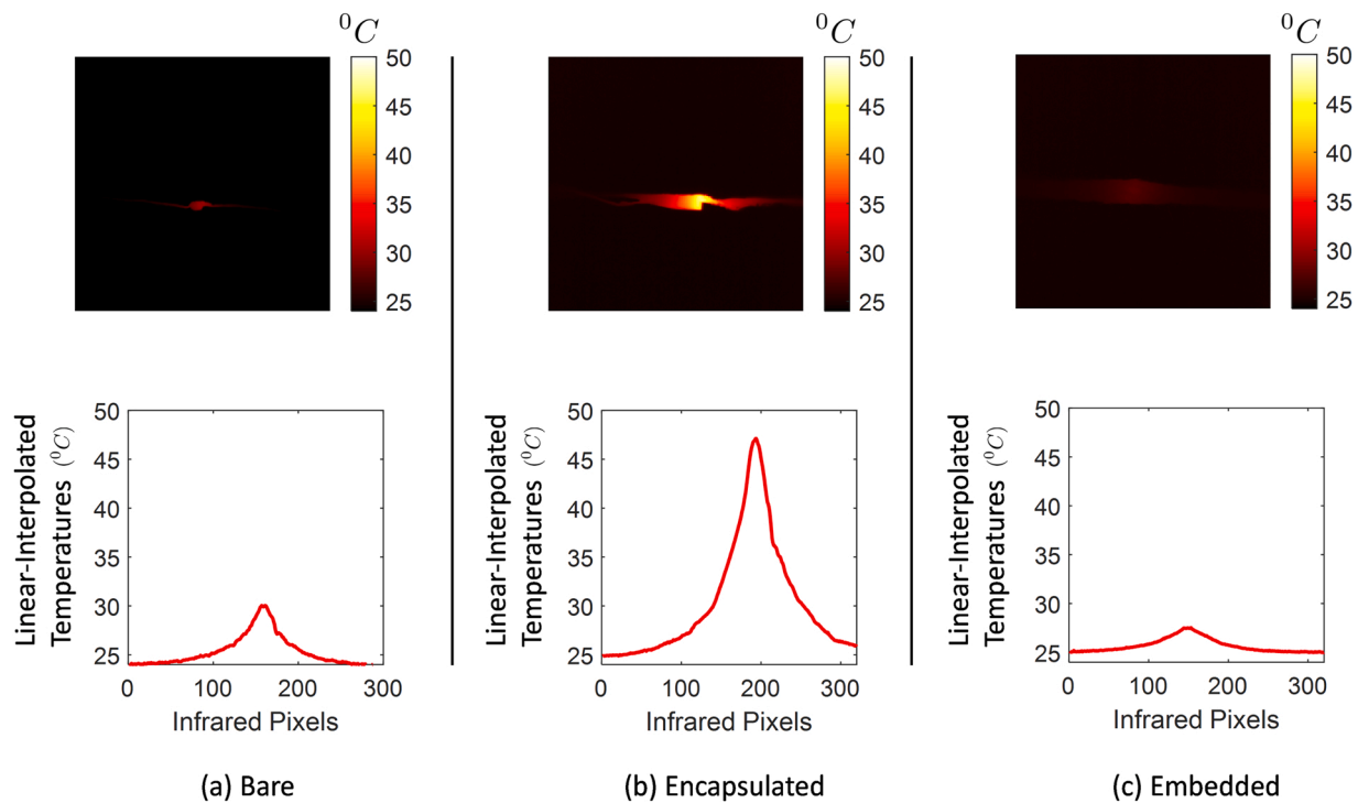
Fig. 7. Linear-interpolated 2D images created by MATLAB for one LED and its corresponding thermal distribution plots based on the temperatures taken from a directly touched thermocouple to a bare (a), encapsulated (b) and embedded (c) LED. All temperatures are in ^{\circ}\text{C} .
