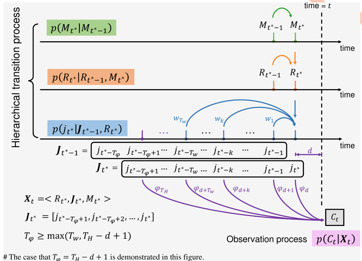
Fig 6. Illustration of the hierarchical transition process and observation process. The most recent infection that can be observed by C_t is at the time t^* = t - d where d is a constant determined by the distribution of observation delay. Suppose T_\varphi is the length of the vector J_{t^*} = [j_{t^*-T_\varphi+1}, j_{t^*-T_\varphi+2}, \dots, j_{t^*}] such that C_t is only relevant to J_{t^*} and j_{t^*} only depends on J_{t^*-1} via the renewal process. Therefore, T_\varphi \geq \max(T_w, T_H - d + 1) . The case that T_\varphi = T_H - d + 1 is depicted in this figure.
