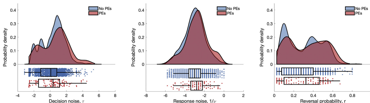
Figure 1. Probability density distributions (top panels) and individual counts with boxplot (bottom panels) of the parameter estimates for decision noise (in the draws-to-decision task) and response noise and reversal probability (in the probability estimation task) shown for participants with (red) and without (blue) psychotic experiences (PEs). The evidence for an association between these parameters and PEs was robust only for decision noise. There was no evidence for an association with response noise after adjusting, and reversal probability showed an association only when treated as a binary measure in the sensitivity analyses.
