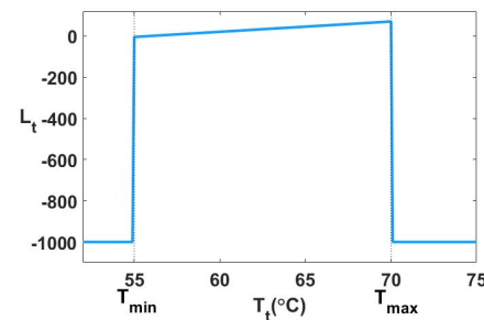
FIGURE 2. Output curve of term L_t for different temperature.
