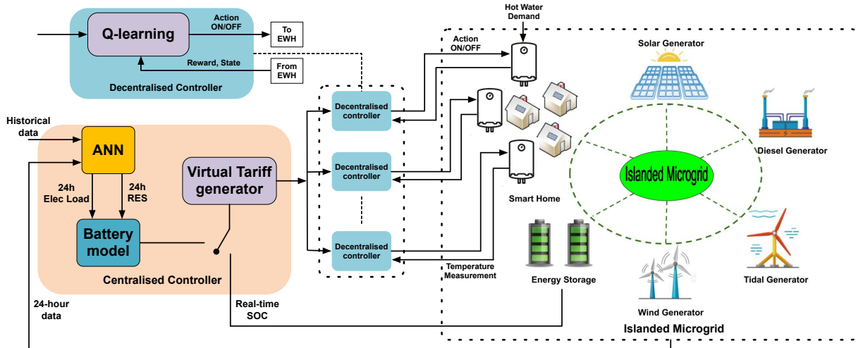
FIGURE 1. Islanded Microgrid and control strategy framework
