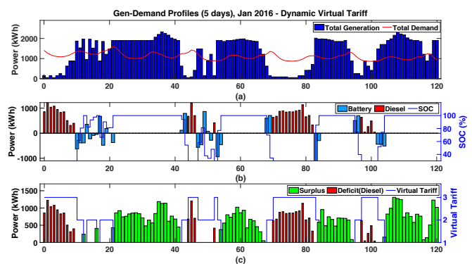
FIGURE 3. Performance of the proposed strategy in Scenario 3.
