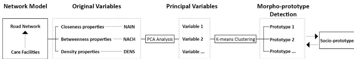
Figure 2. Methodology framework
