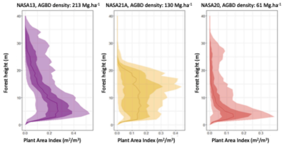
Fig. 2. Plant area volume density as a function of canopy height in three plots in Mondah forest (plot 13, 21 and 20). The lightest shade is 0.1–0.9 percentile, the darker shade is 0.3–0.7 percentile and the line is the 0.5 quantile.
