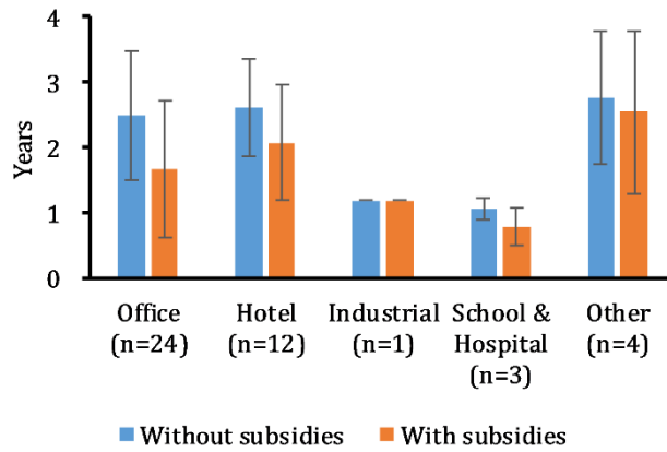
Fig. 4. Payback periods by building types (EE retrofit). Error bars refer to the standard deviation of each set.
