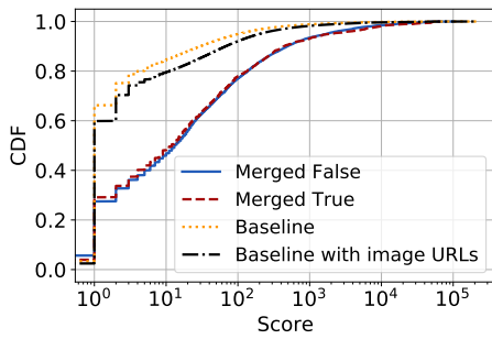
Figure 8: CDF of Reddit submission score on submissions sharing directly images.
