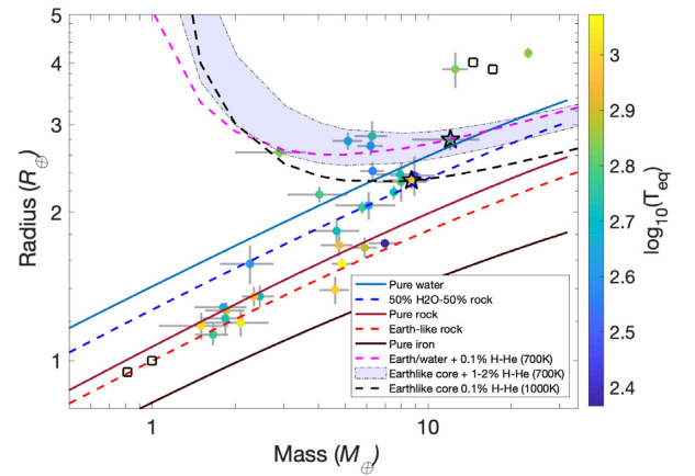
Figure 10. Mass-radius diagram of planets with measured masses better than 30 per cent and radii better than 10 per cent orbiting mid-M to mid-K dwarfs (3000–4400 K). In total there are 26 planets in 19 multiplanet systems. Models of core compositions without atmosphere (Zeng et al. 2016) and with atmosphere (Zeng et al. 2019) at different equilibrium temperatures are also plotted. TOI-1260 b and TOI-1260 c are marked with star symbols, and squares are the Solar system planets.
