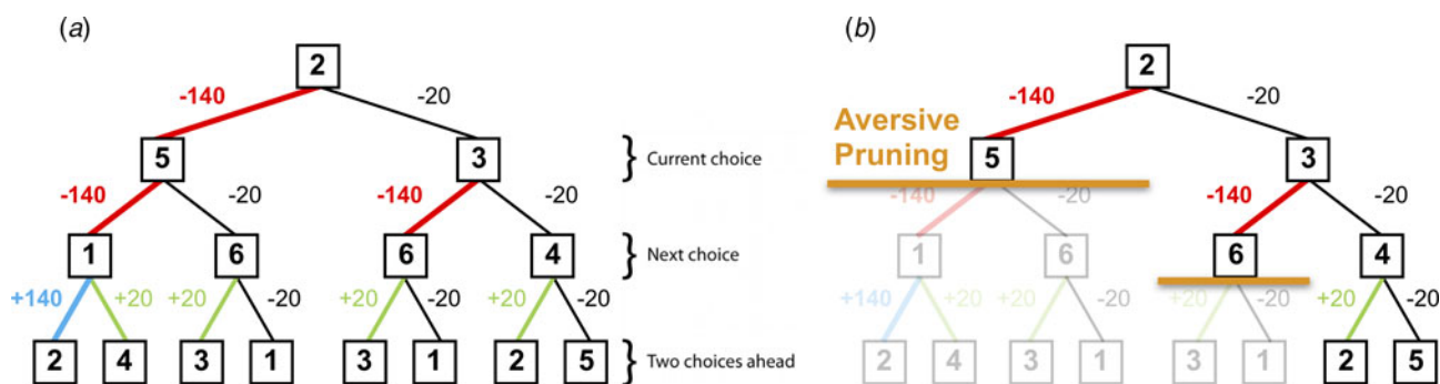
Fig. 2. (a) A typical decision-tree and financial outcomes up to a depth of 3 starting from state 2. Numbers in each box denote the state number. (b) Same decision-tree starting, aversively pruned due to a large negative outcome at the first step. Note that this aversive pruning also avoids the large positive transition, but almost halves the computational load.
