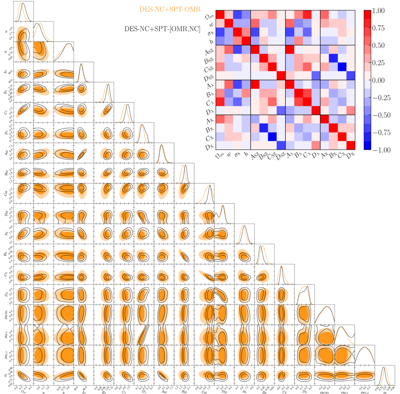
FIG. 13. Marginalized posterior distributions for the w\Lambda\text{CDM} + \sum m_\nu model. The 2D contours correspond to the 68% and 95% confidence levels of the marginalized posterior distribution. The description of the model parameters along with their posteriors are listed in Table III. Inset panel : Correlation matrix for the scaling relations and cosmological parameters derived from the DES-NC + SPT-OMR analysis.
