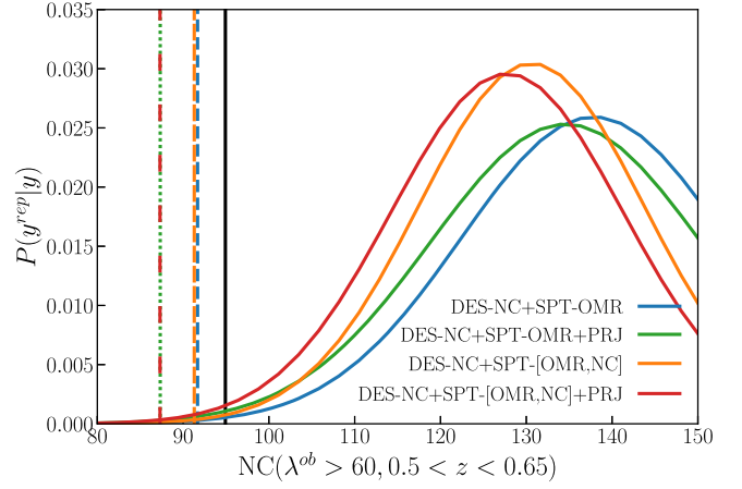
FIG. 6. Posterior predictive distributions for the highest- \lambda/z data point derived from the four analyses considered in Sec. IV A. The solid black line correspond to the observed cluster abundance in that bin, while the four dashed and dot-dashed lines mark the 3\sigma limit of the corresponding posterior predictive distribution. Although residing in the tail of the distributions, in none of the four analyses the observed data point lies outside the 3\sigma region.
