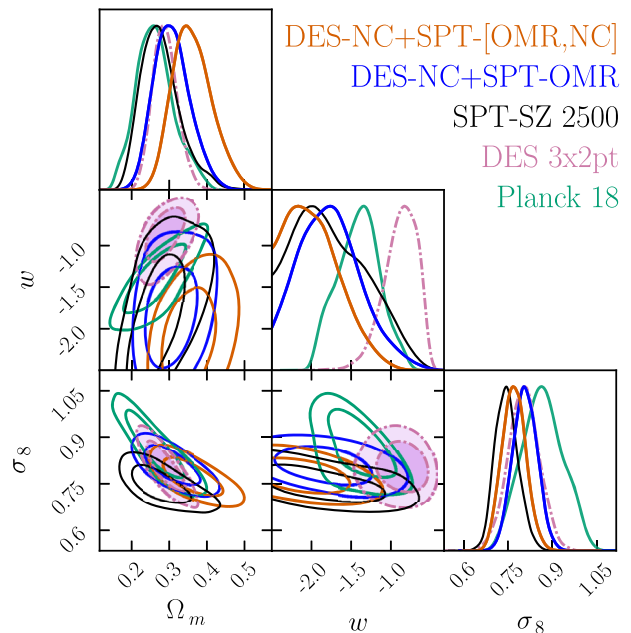
FIG. 11. Cosmological posteriors (68% and 95% C.L.) for the w\text{CDM} + \sum m_\nu model from the combination of DES-NC and SPT-OMR data (blue) and the full data combination (orange). For comparison we include in the figure the posteriors obtained from Planck CMB (green), DES 3x2pt (pink) and SPT-SZ 2500 (black) analyses.
