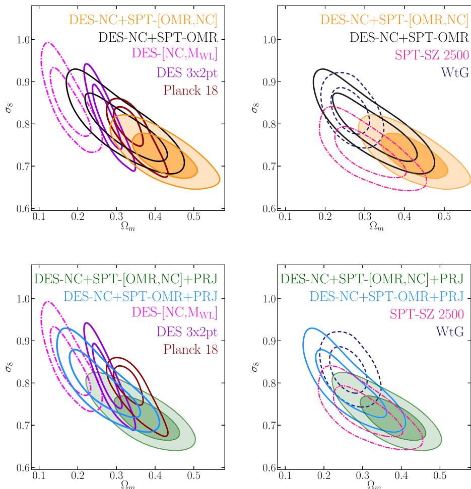
FIG. 7. Upper panels : Comparison of the 68% and 95% confidence contours in the \sigma_8 - \Omega_m plane derived in this work adopting the BKG scatter model ( black and orange contours ) with other constraints from the literature: DES Y1 cluster counts and weak lensing mass calibration [DES20, dot-dashed magenta contours ]; DES-Y1 3x2 from [ [49], dark violet contours ]; Planck CMB from [ [40], brown contours ]; cluster number counts and follow-up data from the SPT-SZ 2500 survey [B19, dot-dashed pink contours ]; cluster abundance analysis of weighing the giants [ [5], WtG, dashed dark blue contours ]. Lower panels : Same as left panel but considering the projection effect model (PRJ) for the scatter between true and observed richness (see Sec. III A).
