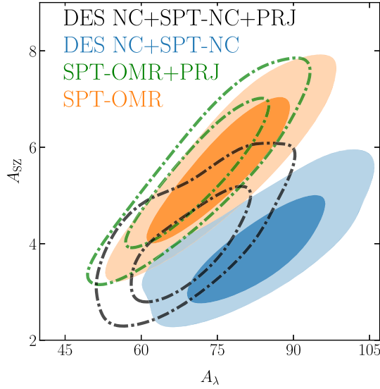
FIG. 8. 68% and 95% confidence contours for the amplitude parameters A_\lambda - A_{SZ} from the combination of DES Y1 and SPT cluster counts data ( blue and black ) or the SPT multiwavelength data ( orange and green ), including ( dot-dashed contours) or not ( filled contours) the projection effect model (PRJ). All the contours are derived imposing the cosmological priors resulting from the combination of the posteriors obtained from the DES-NC + SPT-OMR and SPT-[OMR,NC] analyses. By shifting the abundance posteriors towards lower A_\lambda values ( black versus blue contours) the PRJ model relieves the tension between the scaling relation parameters preferred by abundance and multiwavelength data.
