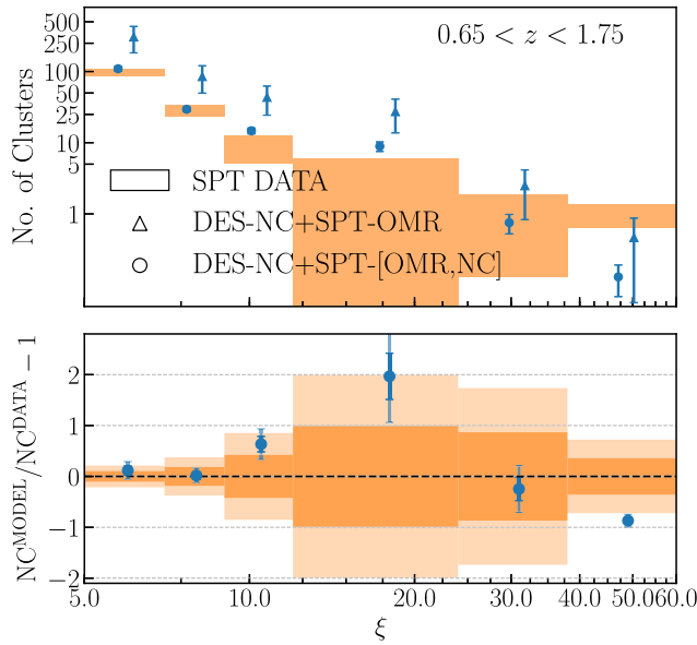
FIG. 5. Observed SPT-SZ cluster number counts ( shaded areas ) and mean model predictions from the DES-NC + SPT-OMR ( triangles ) and DES-NC + SPT-[OMR, NC] ( circles ) analyses, as a function of \xi . The points have been slightly displaced along the \xi axis to avoid overcrowding. The y extent of the data boxes corresponds to the Poisson noise. The bottom panel shows the residual between the data and the mean model predictions derived from DES-NC + SPT-[OMR, NC]. The error bars on the predicted number counts represent 1 and 2 standard deviations of the distribution derived sampling the relevant parameters of the corresponding chain. The y extent of the data boxes corresponds to 1 and 2 standard deviations of the associated Poisson distribution. The SPT-NC model predictions for the two analyses including the PRJ model are fully consistent with those obtained from the baseline model and thus not included in the plot to avoid overcrowding.
