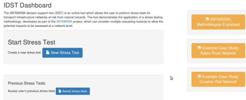
Figure 2 IDST Dashboard
