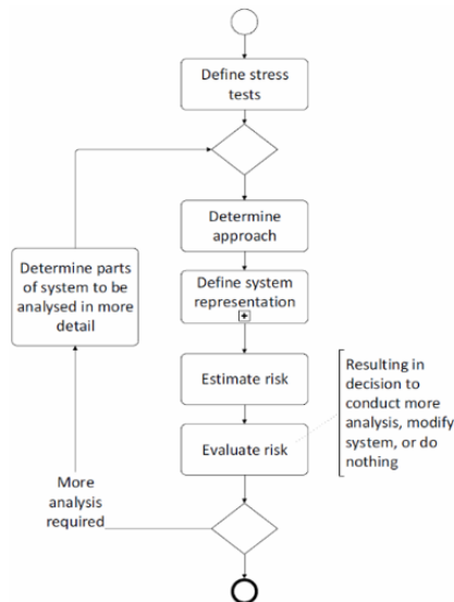
Figure 3 IDST Workflow
