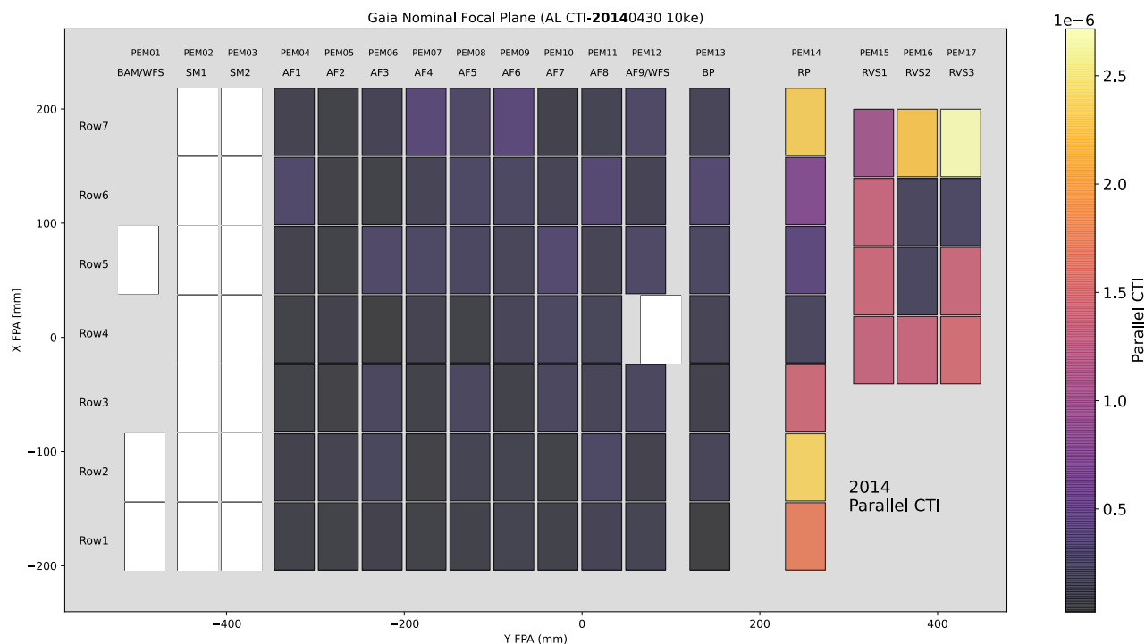
Figure 4. The distribution of the parallel CTI values, at a signal of 10 000 electrons, across the focal plane as measured from the data in April 2014. A comparison of this Figure with Figure 2 reveals that the devices manufactured in 2009 have a higher initial CTI
