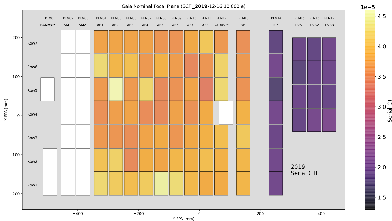
Figure 5. The distribution of the serial CTI (at 10 000 electrons) across the focal plane as measured in December 2019.
