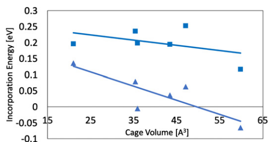
Figure 3. The highest (squares) and lowest (triangles) incorporation energies for interstitials that are found in the cages as determined by the Voronoi–Delaunay tessellation analysis. This energy dependence is based on the orientation of the molecule with respect to the cage.
