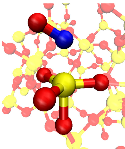
Figure 6. The majority interaction of the \text{NO}^- . The N interacts with the \text{SiO}_4 tetrahedron, akin to the negative NO in the literature, flattening a face of the tetrahedron. Color coding is the same as figure 5.
