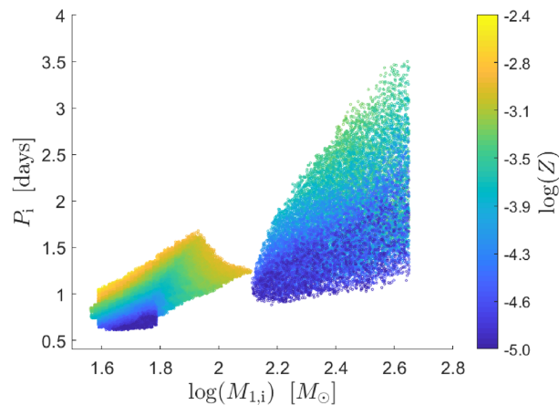
Figure 6. The distribution of initial masses and initial periods for systems that will produce BHBH systems merging within the lifetime of the Universe, where the colour indicates the metallicity. The trend towards longer periods at higher masses can also be seen from the grids in Appendix A.
