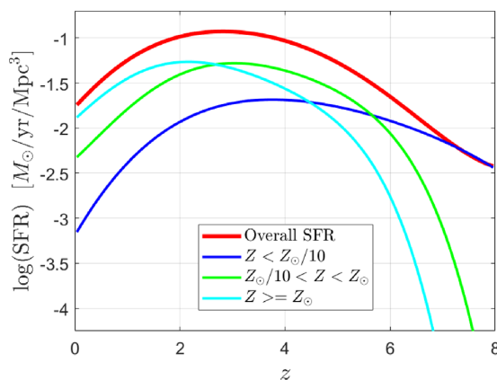
Figure 2. The Madau plot shown for different ranges of metallicity for the hydrodynamical simulations of Taylor & Kobayashi (2015a), discussed in Section 2.1. Red: The Madau plot for all ranges of metallicity; Dark blue: For metallicities Z < Z_\odot/10 ; Green: Z_\odot/10 < Z < Z_\odot ; Light blue: Z \geq Z_\odot . For this work, solar metallicity Z_\odot is taken to be 0.017 as in Grevesse et al. (1996). For the metallicity range considered in our Monte Carlo simulation ( -5.0 < \log(Z) < -2.375 , as discussed in Section 2.3), the dark blue and green curves are the only relevant curves.
