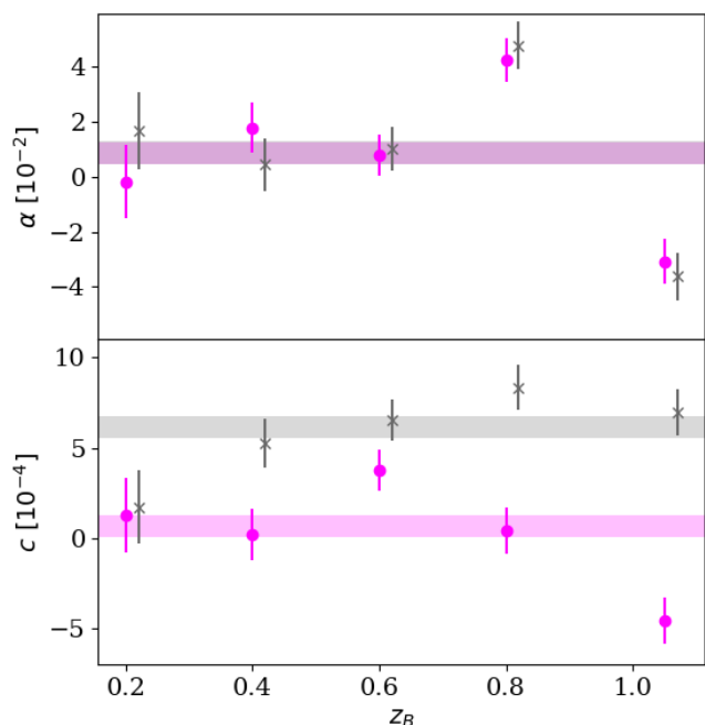
Fig. 6: Systematics parameters: the amplitude of the PSF residual fraction \alpha , and the additive parameter c , from Eq. (12), as a function of tomographic photometric redshift bin, z_B . The tomographic measurements can be compared per ellipticity component, \epsilon_1 (closed, pink) and \epsilon_2 (crosses, grey), and with a non-tomographic measurement (shown as coloured grey/pink bars of width 1\sigma ).
