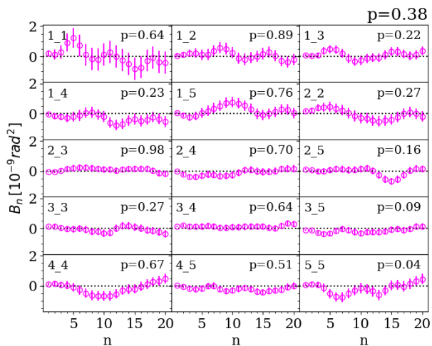
Fig. 9: KiDS-1000 B-mode null-test: the COSEBIs B_n modes are shown for each tomographic bin combination (denoted in the upper left corner of each panel). The measured B-modes are consistent with random noise, as determined through the p -values shown in the upper right corner of each panel. Considering the full data vector of n = 20 modes and 15 different tomographic bin combinations, we find p = 0.38 corresponding to an insignificant 0.3\sigma deviation from a null signal. We caution the reader against ‘chi-by-eye’ as the B_n modes are highly correlated.
