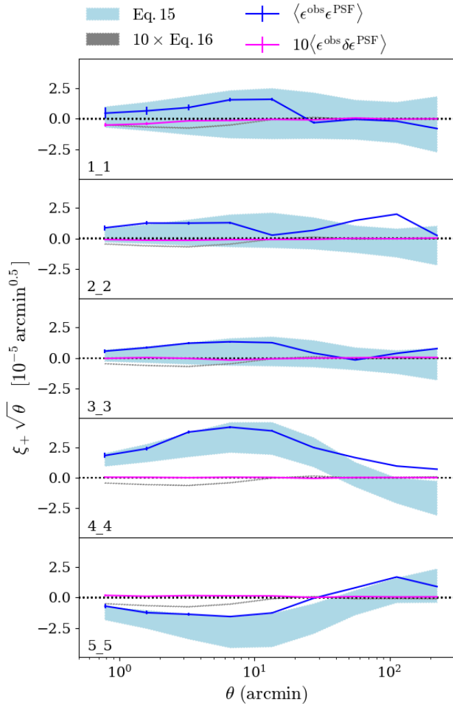
Fig. 7: Comparison of two star-galaxy cross-correlation functions with their corresponding linear systematics model predictions (Eqs. 15 and 16) for the five tomographic bins. The star-galaxy cross correlation function \langle \epsilon_{\text{corr}}^{\text{obs}} \epsilon^{\text{PSF}} \rangle (dark blue) is in reasonable agreement with the model (blue bar), where the width of the model reflects the 2\sigma uncertainty. The residual star-galaxy cross correlation function \langle \epsilon_{\text{corr}}^{\text{obs}} \delta \epsilon^{\text{PSF}} \rangle (shown pink), and corresponding model (grey), are scaled by a factor of ten in order to display the measurements on the same scale. We also scale the correlation functions by \sqrt{\theta} to aid visualisation of the large-scale signal.
