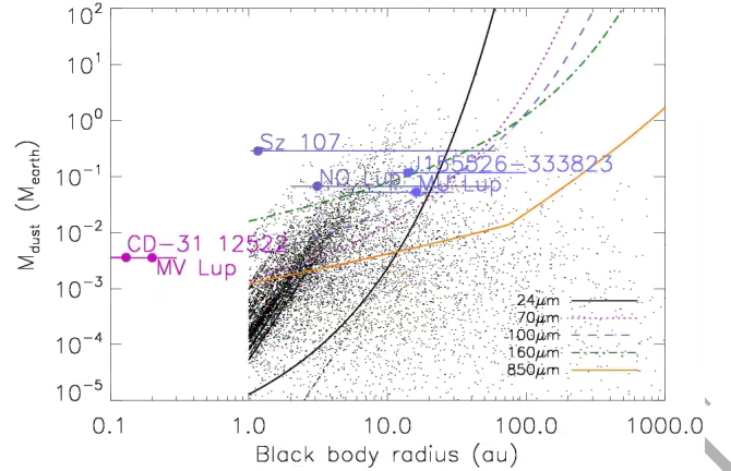
Figure 14. Top: Predicted population dust mass and radii for a sample of 10,000 disks based on the models of Wyatt et al. (2007) ; Sibthorpe et al. (2018) , and the expected detection thresholds at 24\mu\text{m} , 70\mu\text{m} (i.e., with Spitzer ), 100\mu\text{m} , 160\mu\text{m} (i.e., with Herschel ) and 850\mu\text{m} (i.e., with ALMA ). Shown are the positions of the 4 sub-mm detections (lilac) and the 2 hot IR-excesses (pink). Note that the plotted radii are approximated by the black body SED fits (based on temperature and fractional luminosity which have a large range of values see Table 4) but that these span a wide range of values consistent with their detections/non-detections with either Spitzer (at 24\mu\text{m} ) or ALMA (at 850\mu\text{m} ).
