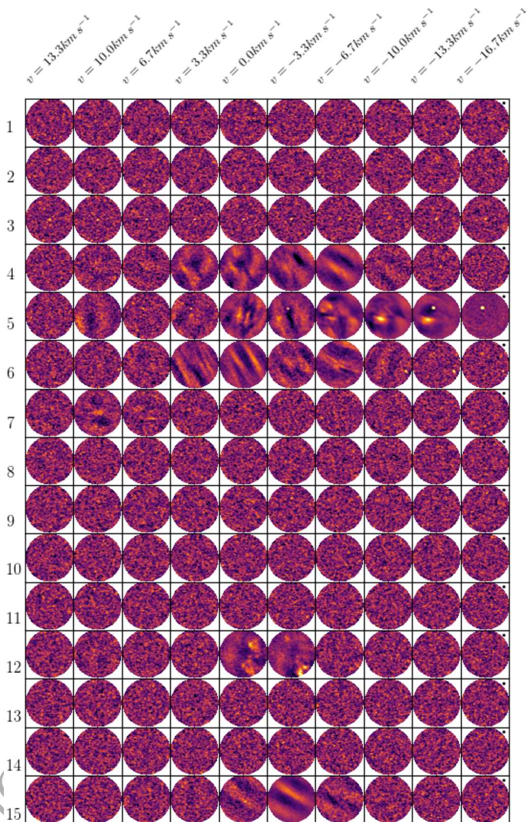
Figure C1. ALMA Channel Maps for target source IDs 1-15. Large scale emission was seen in sources 4, 5, 6, 7, 12 and 15 (prior to removing all baselines < 100k\lambda ) assumed to be cloud emission from Lupus. In all images, North is up, East is left, and the beam is shown in the upper right of the right-most panel for each source. CO emission can be seen clearly in source 3 and 5, and towards the South East of source 6 for velocities v < -6.7 \text{ km s}^{-1} .
