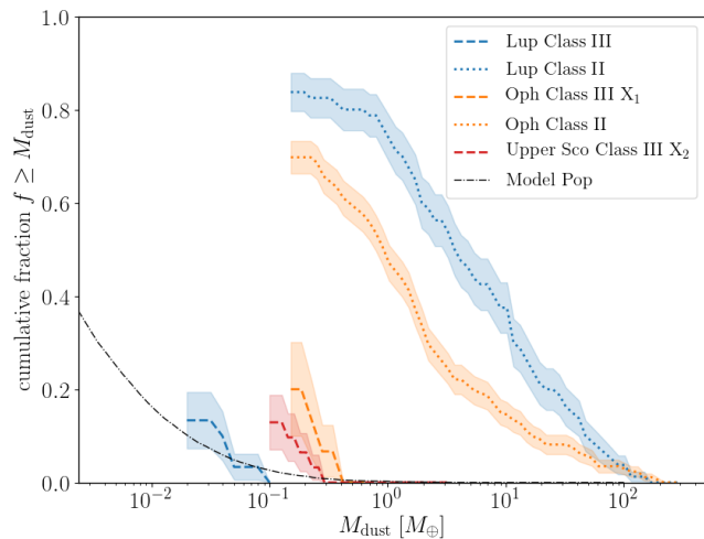
Figure 13. Cumulative fraction of disks with a mass greater than those in the binned range for Lupus sources (blue), where class III are dashed and class II are dotted, and similarly for Ophiuchus (in orange) and class III sources in Upper Sco (in red), noting that for both Ophiuchus and Upper Sco the class III sources were selected based on different constraints to our Lupus survey, and are hence labelled as Class III X 1 or Class III X 2 here. The shaded regions represent 1\sigma confidence intervals.
