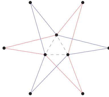
FIGURE 5 Applying Theorem 3.8 gives many copies of H \odot_2 (H, h) in which the central copy of H is green-forced [Colour figure can be viewed at wileyonlinelibrary.com ]
