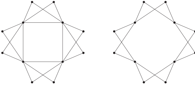
FIGURE 1 C_4 \ominus_2 K_3 (on the left) and C_4 \odot_2 K_3 (on the right)
