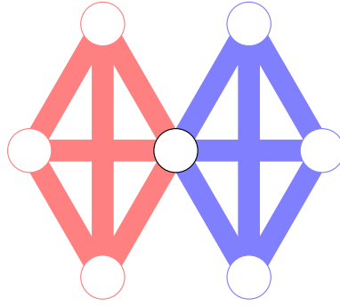
FIGURE 2 The parts of G corresponding to the two cliques from Corollary 3.10 [Colour figure can be viewed at wileyonlinelibrary.com ]
