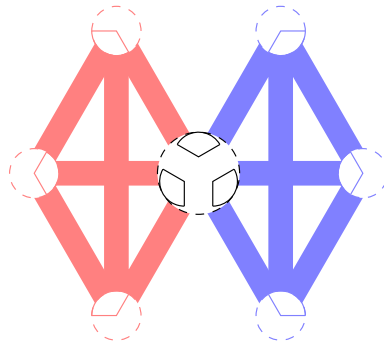
FIGURE 3 We divide the central part into v(H) subsets and shrink the other parts accordingly [Colour figure can be viewed at wileyonlinelibrary.com ]
