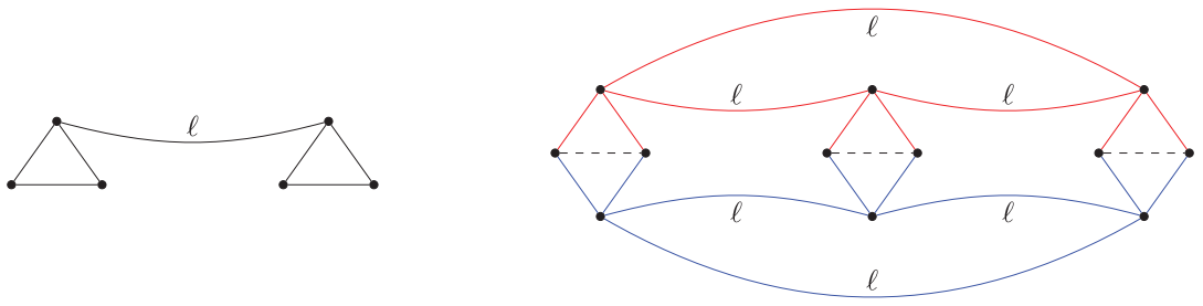
FIGURE 6 H , drawn on the left, consists of two triangles joined by a path of length \ell . On the right, F_{red} is drawn in red, F_{blue} in blue and the matching M is drawn with dashed lines [Colour figure can be viewed at wileyonlinelibrary.com]
