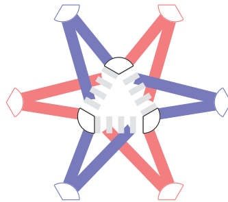
FIGURE 4 We imagine a copy of H between the subsets of the central part, with each edge supporting both a red and a blue copy of H \setminus h using the parts from the red and blue cliques [Colour figure can be viewed at wileyonlinelibrary.com ]
